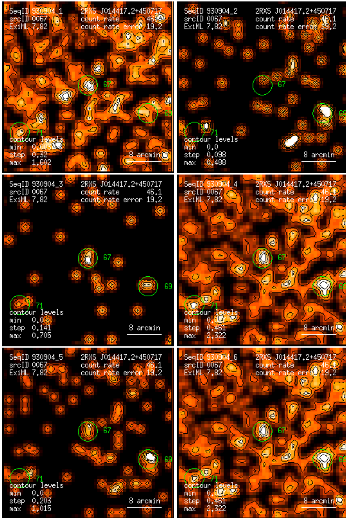
Figure 67: RASS 930904: detection 0067: band rate images, Gaussian filter: (1) PSPC channels 11 – 41, (2) 52 – 90, (3) 91 – 201, (4) 11 – 235, (5) 52 – 201, (6) 11 – 201. Broad band rates in counts/ks. Band rate contour levels in counts/ks/arcmin 2 .
