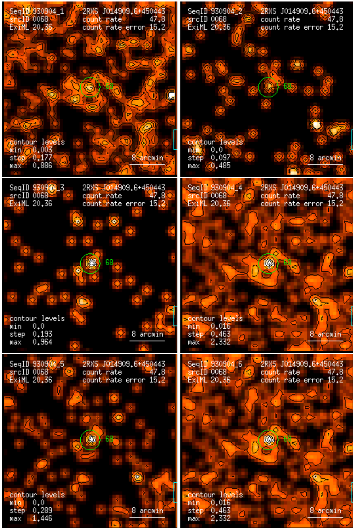
Figure 68: RASS 930904: detection 0068: band rate images, Gaussian filter: (1) PSPC channels 11 – 41, (2) 52 – 90, (3) 91 – 201, (4) 11 – 235, (5) 52 – 201, (6) 11 – 201. Broad band rates in counts/ks. Band rate contour levels in counts/ks/arcmin 2 .
