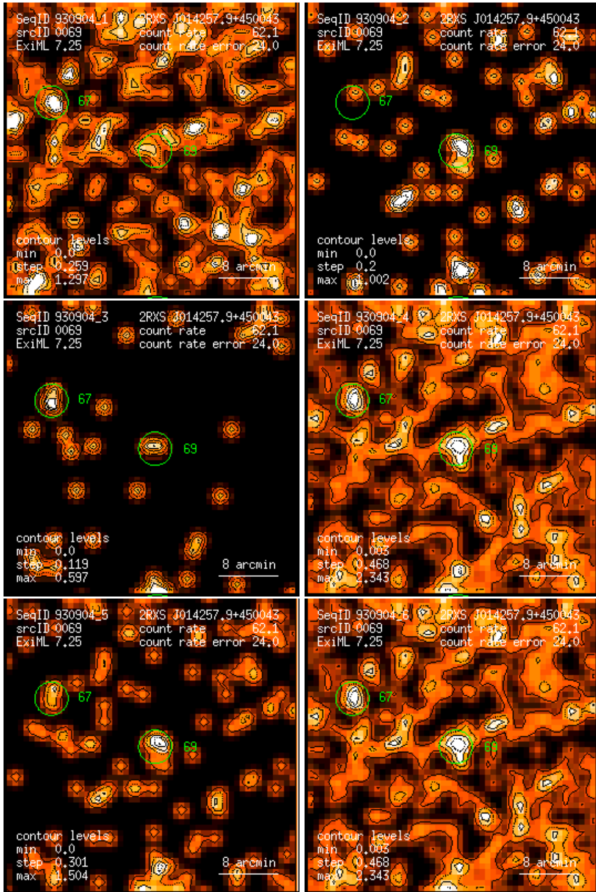
Figure 69: RASS 930904: detection 0069: band rate images, Gaussian filter: (1) PSPC channels 11 – 41, (2) 52 – 90, (3) 91 – 201, (4) 11 – 235, (5) 52 – 201, (6) 11 – 201. Broad band rates in counts/ks. Band rate contour levels in counts/ks/arcmin 2 .
