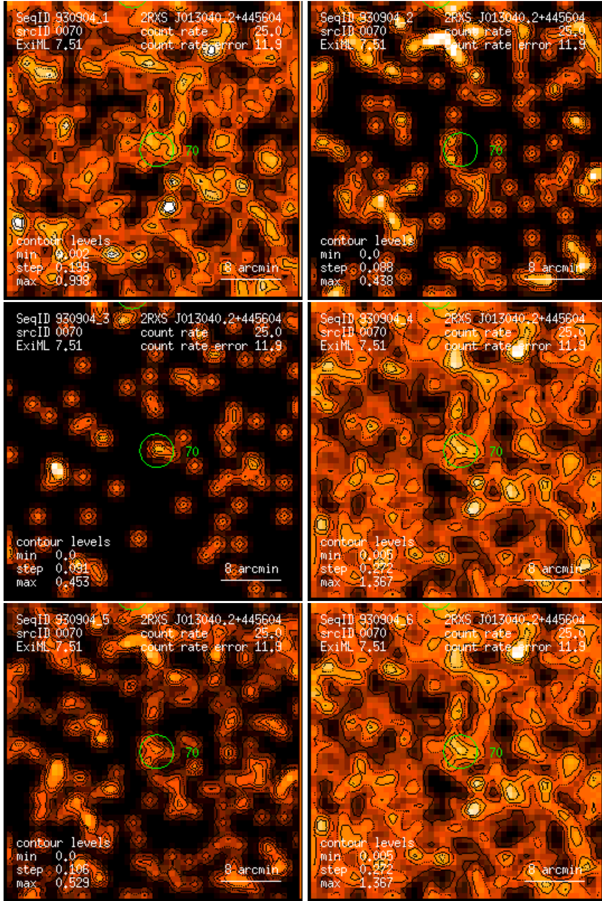
Figure 70: RASS 930904: detection 0070: band rate images, Gaussian filter: (1) PSPC channels 11 – 41, (2) 52 – 90, (3) 91 – 201, (4) 11 – 235, (5) 52 – 201, (6) 11 – 201. Broad band rates in counts/ks. Band rate contour levels in counts/ks/arcmin 2 .
