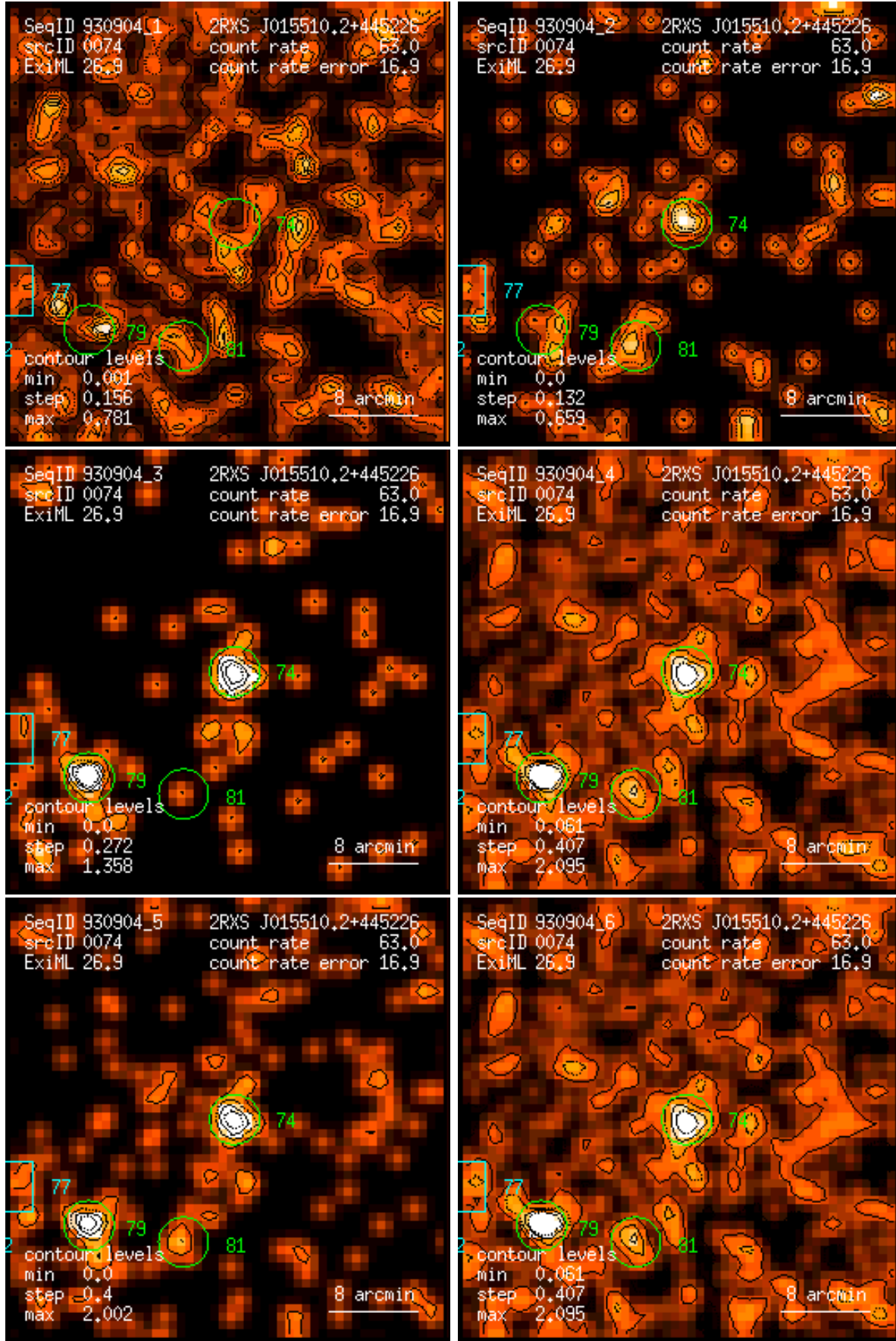
Figure 74: RASS 930904: detection 0074: band rate images, Gaussian filter: (1) PSPC channels 11 – 41, (2) 52 – 90, (3) 91 – 201, (4) 11 – 235, (5) 52 – 201, (6) 11 – 201. Broad band rates in counts/ks. Band rate contour levels in counts/ks/arcmin 2 .
