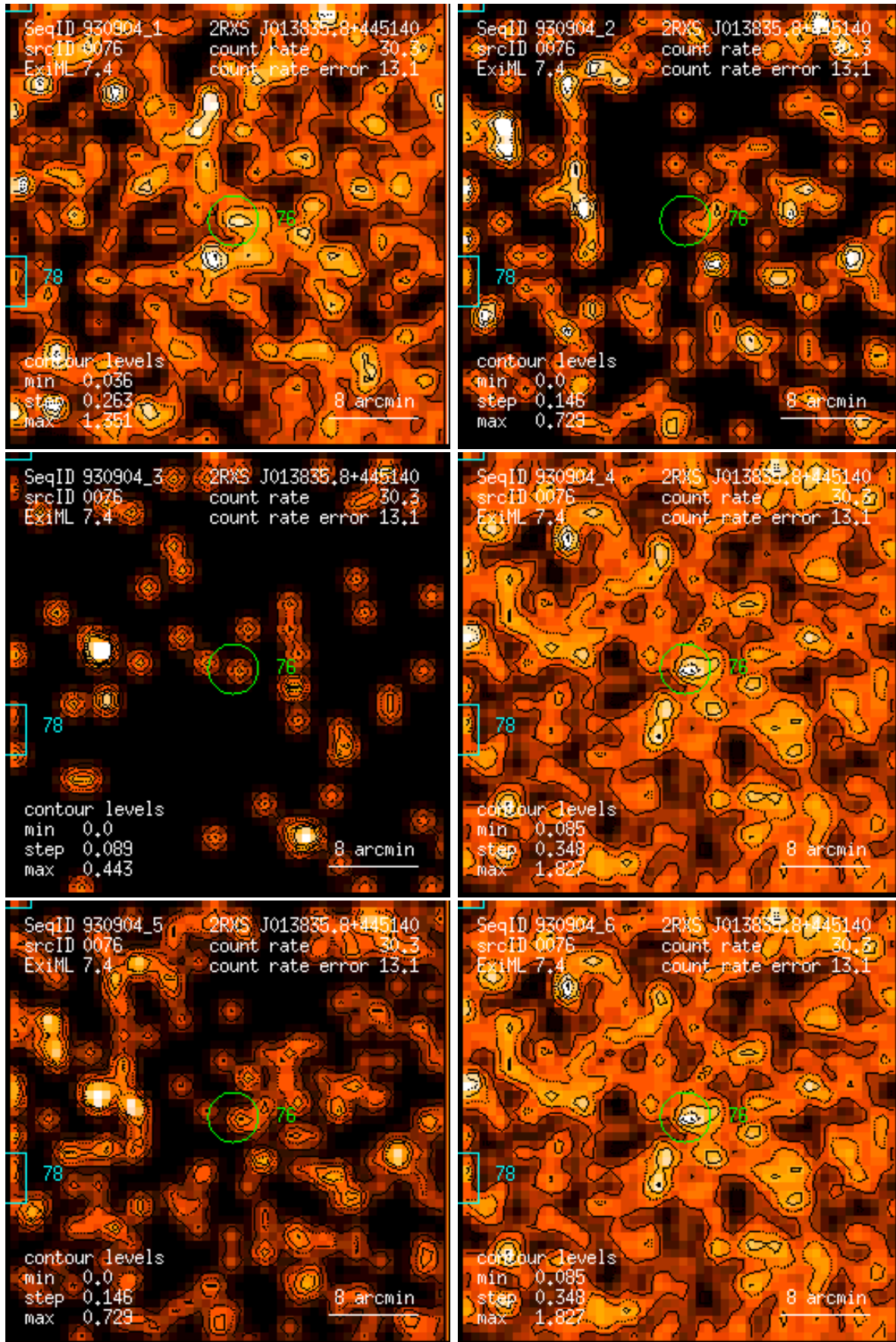
Figure 76: RASS 930904: detection 0076: band rate images, Gaussian filter: (1) PSPC channels 11 – 41, (2) 52 – 90, (3) 91 – 201, (4) 11 – 235, (5) 52 – 201, (6) 11 – 201. Broad band rates in counts/ks. Band rate contour levels in counts/ks/arcmin 2 .
