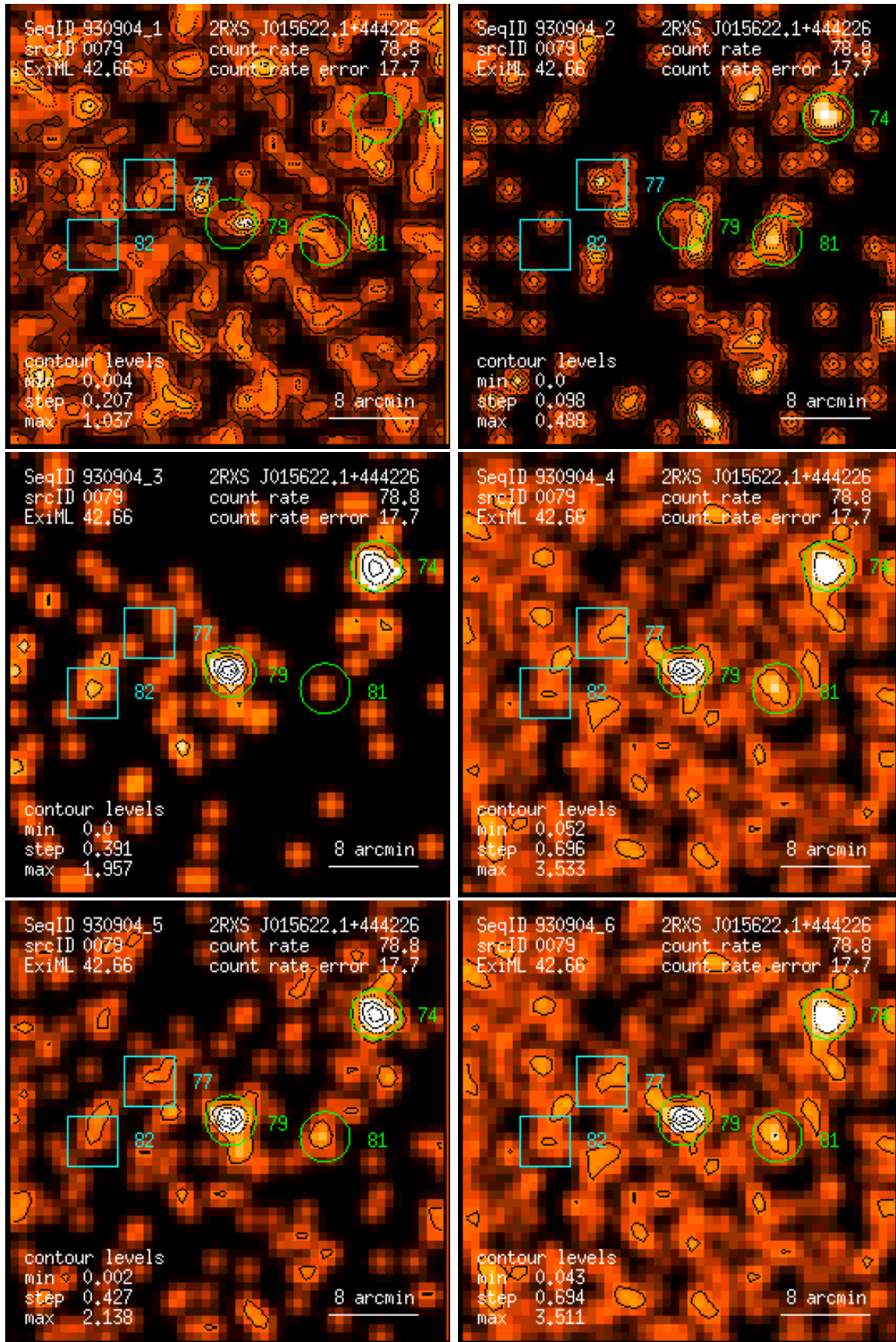
Figure 79: RASS 930904: detection 0079: band rate images, Gaussian filter: (1) PSPC channels 11 – 41, (2) 52 – 90, (3) 91 – 201, (4) 11 – 235, (5) 52 – 201, (6) 11 – 201. Broad band rates in counts/ks. Band rate contour levels in counts/ks/arcmin 2 .
