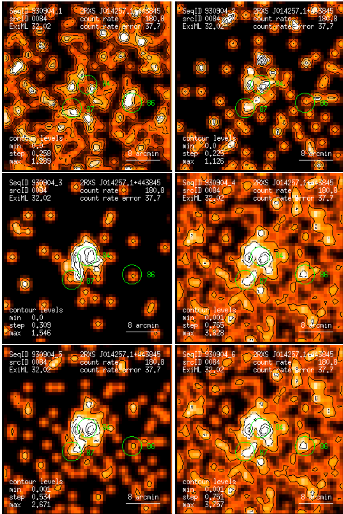
Figure 84: RASS 930904: detection 0084: band rate images, Gaussian filter: (1) PSPC channels 11 – 41, (2) 52 – 90, (3) 91 – 201, (4) 11 – 235, (5) 52 – 201, (6) 11 – 201. Broad band rates in counts/ks. Band rate contour levels in counts/ks/arcmin 2 .
