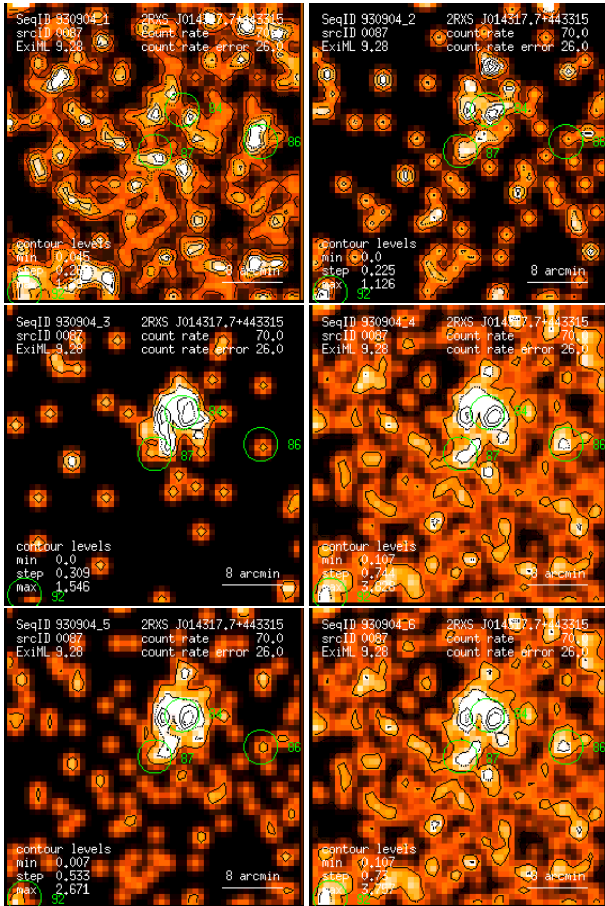
Figure 87: RASS 930904: detection 0087: band rate images, Gaussian filter: (1) PSPC channels 11 – 41, (2) 52 – 90, (3) 91 – 201, (4) 11 – 235, (5) 52 – 201, (6) 11 – 201. Broad band rates in counts/ks. Band rate contour levels in counts/ks/arcmin 2 .
