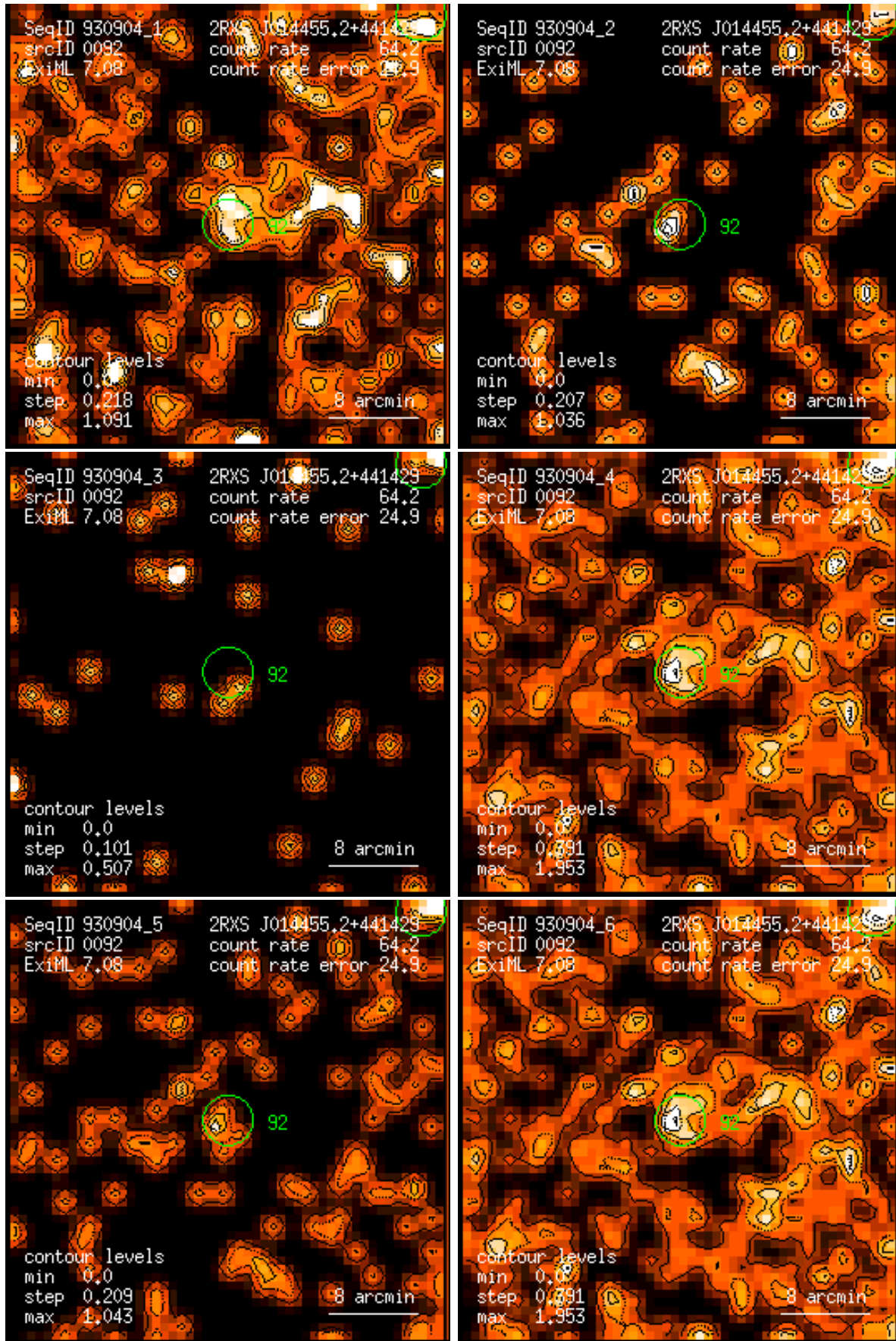
Figure 92: RASS 930904: detection 0092: band rate images, Gaussian filter: (1) PSPC channels 11 – 41, (2) 52 – 90, (3) 91 – 201, (4) 11 – 235, (5) 52 – 201, (6) 11 – 201. Broad band rates in counts/ks. Band rate contour levels in counts/ks/arcmin 2 .
