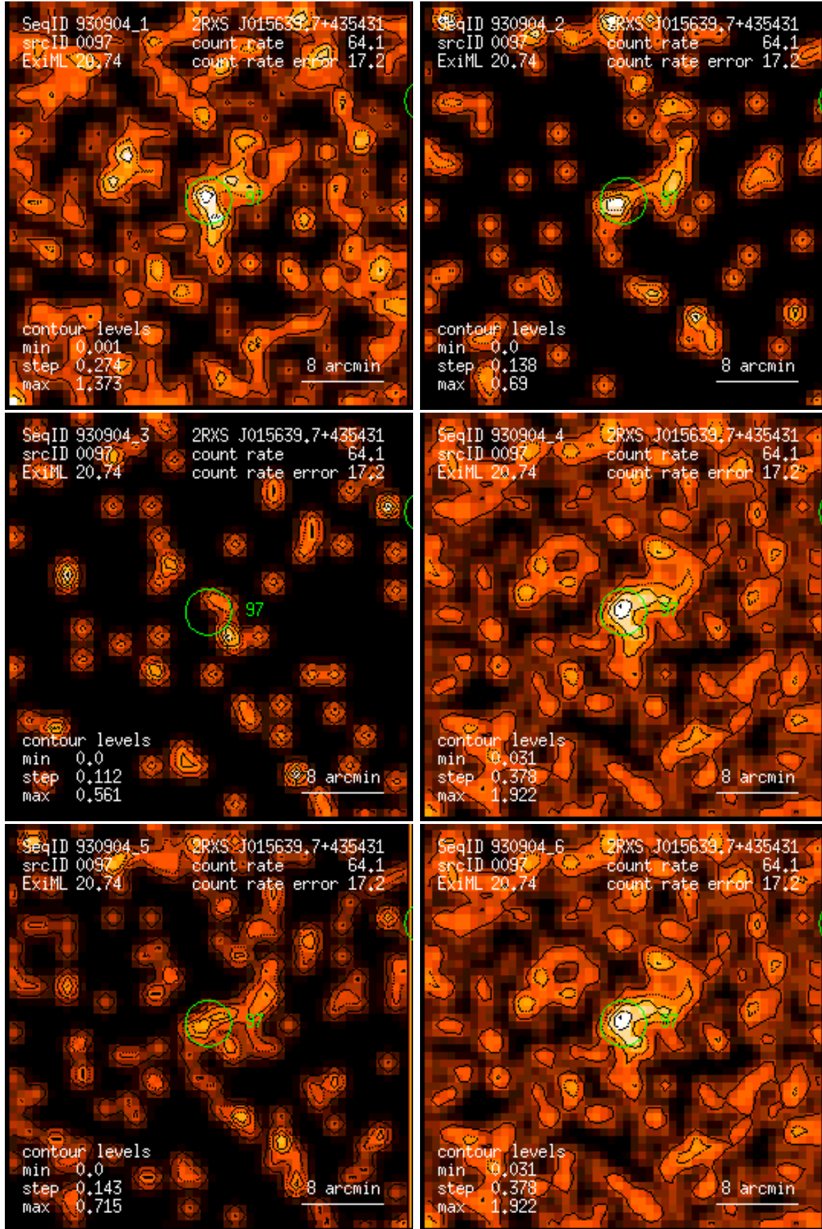
Figure 97: RASS 930904: detection 0097: band rate images, Gaussian filter: (1) PSPC channels 11 – 41, (2) 52 – 90, (3) 91 – 201, (4) 11 – 235, (5) 52 – 201, (6) 11 – 201. Broad band rates in counts/ks. Band rate contour levels in counts/ks/arcmin 2 .
