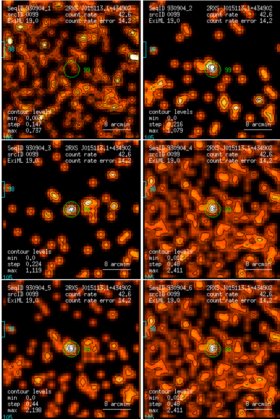
Figure 99: RASS 930904: detection 0099: band rate images, Gaussian filter: (1) PSPC channels 11 – 41, (2) 52 – 90, (3) 91 – 201, (4) 11 – 235, (5) 52 – 201, (6) 11 – 201. Broad band rates in counts/ks. Band rate contour levels in counts/ks/arcmin 2 .
