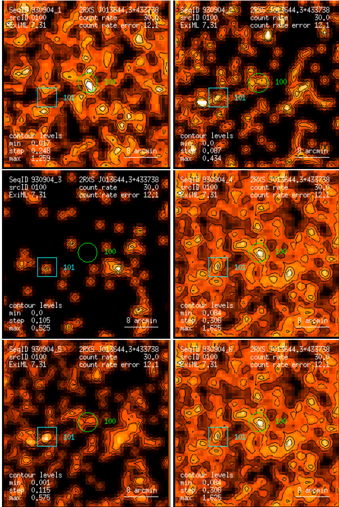
Figure 100: RASS 930904: detection 0100: band rate images, Gaussian filter: (1) PSPC channels 11 – 41, (2) 52 – 90, (3) 91 – 201, (4) 11 – 235, (5) 52 – 201, (6) 11 – 201. Broad band rates in counts/ks. Band rate contour levels in counts/ks/arcmin 2 .
