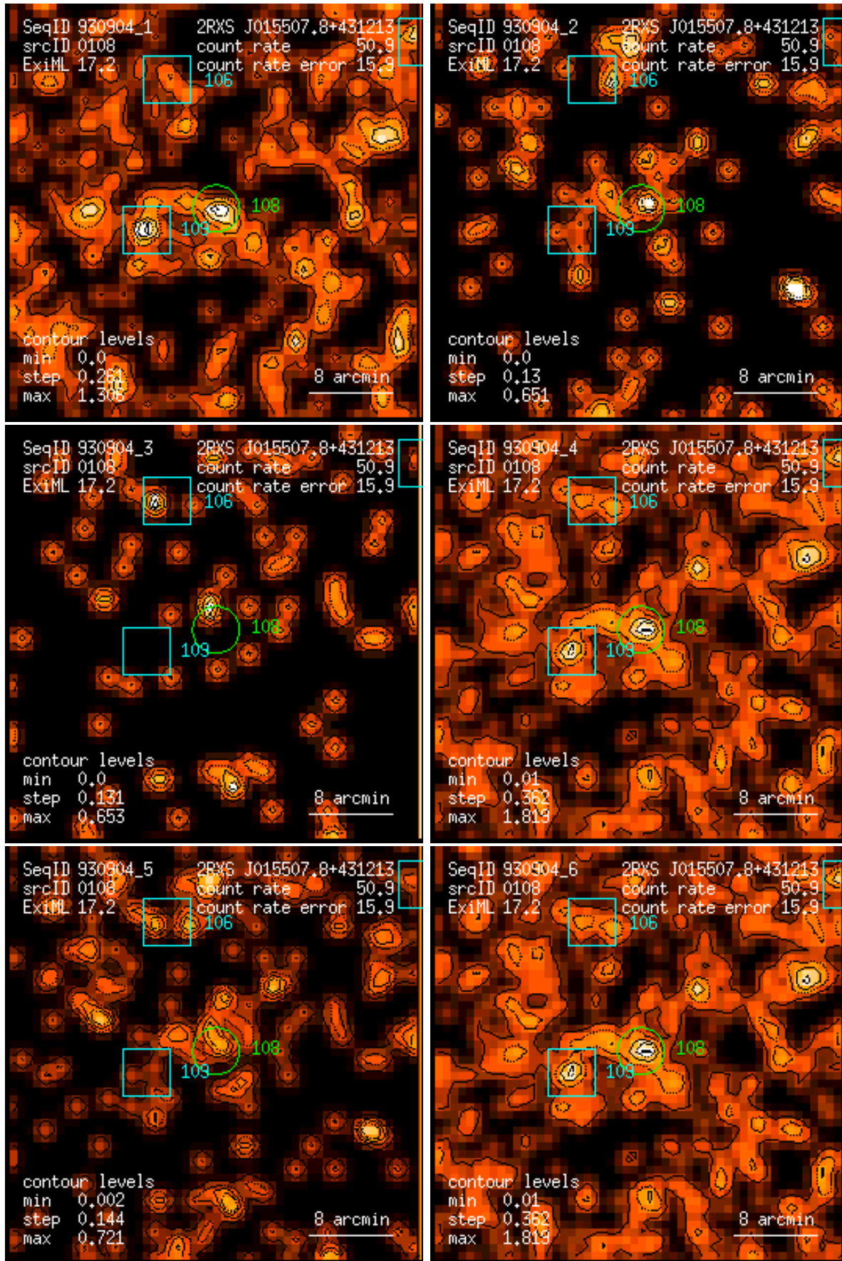
Figure 108: RASS 930904: detection 0108: band rate images, Gaussian filter: (1) PSPC channels 11 – 41, (2) 52 – 90, (3) 91 – 201, (4) 11 – 235, (5) 52 – 201, (6) 11 – 201. Broad band rates in counts/ks. Band rate contour levels in counts/ks/arcmin 2 .
