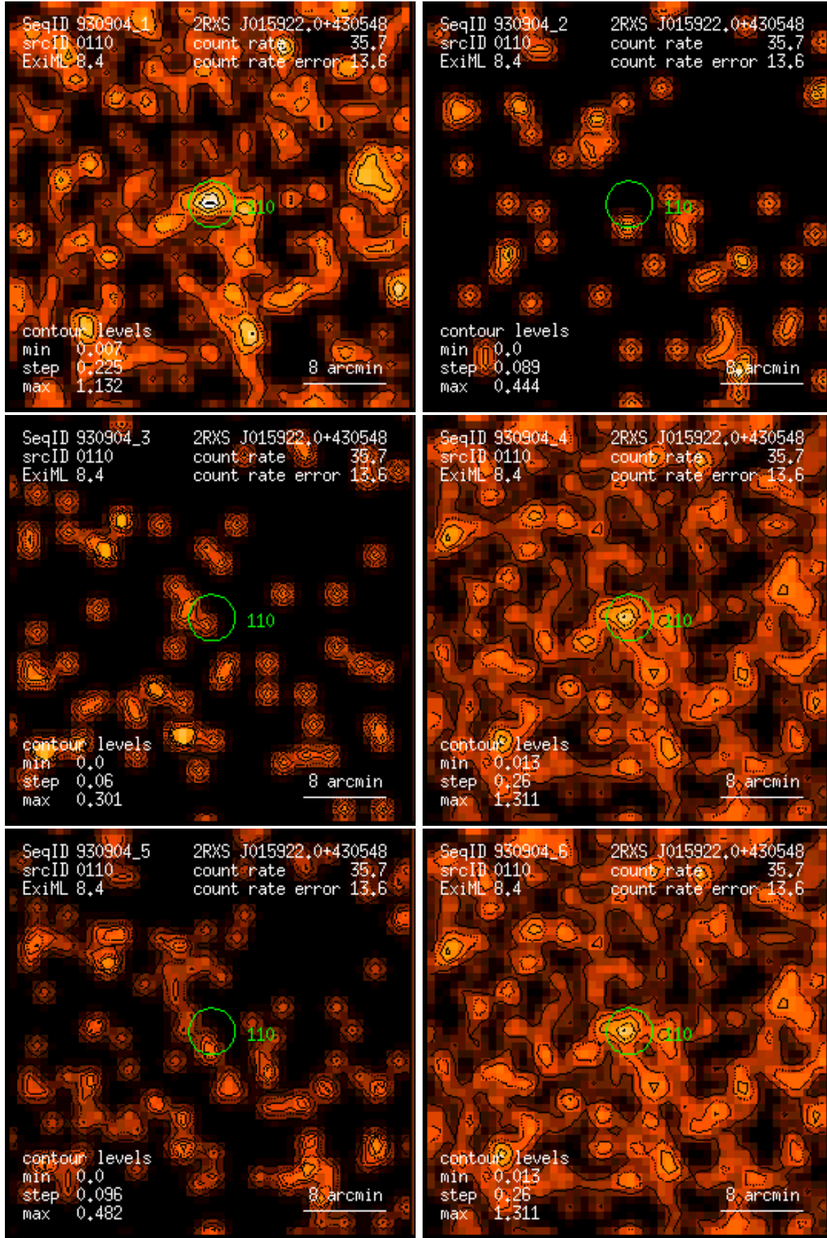
Figure 110: RASS 930904: detection 0110: band rate images, Gaussian filter: (1) PSPC channels 11 – 41, (2) 52 – 90, (3) 91 – 201, (4) 11 – 235, (5) 52 – 201, (6) 11 – 201. Broad band rates in counts/ks. Band rate contour levels in counts/ks/arcmin 2 .
