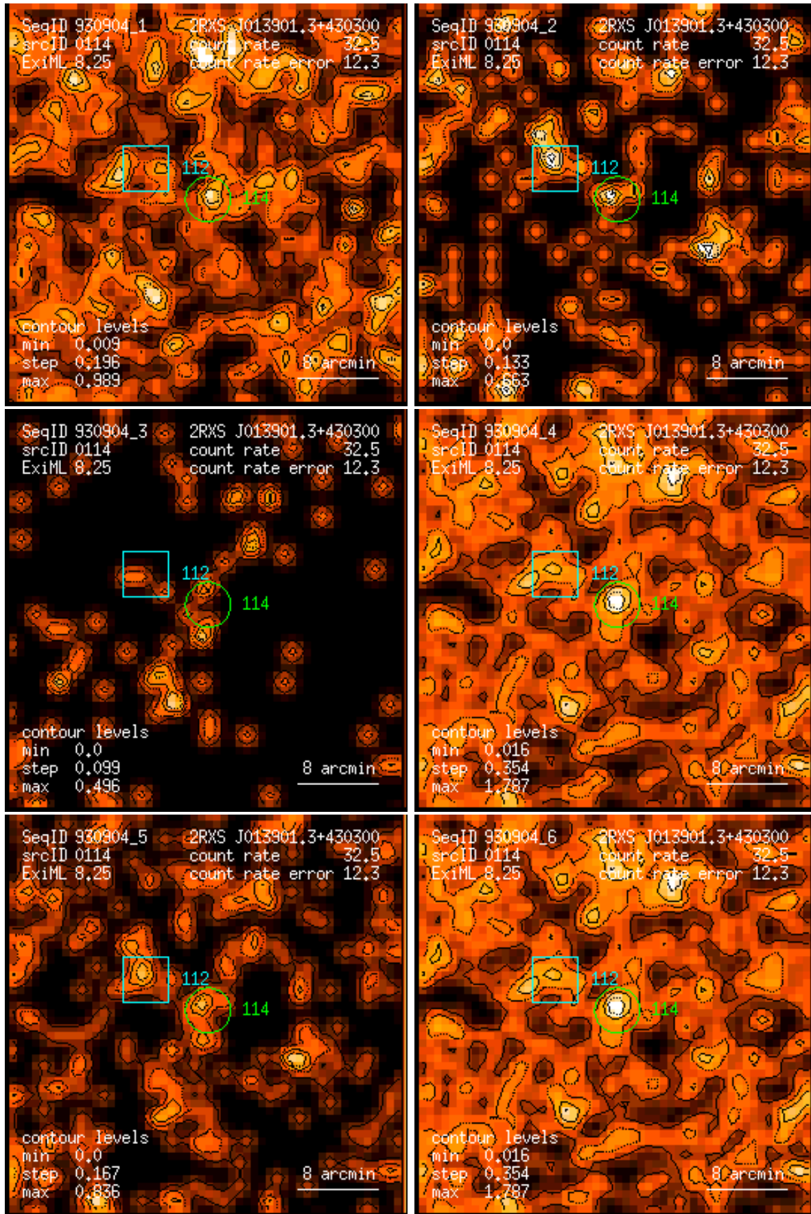
Figure 114: RASS 930904: detection 0114: band rate images, Gaussian filter: (1) PSPC channels 11 – 41, (2) 52 – 90, (3) 91 – 201, (4) 11 – 235, (5) 52 – 201, (6) 11 – 201. Broad band rates in counts/ks. Band rate contour levels in counts/ks/arcmin 2 .
