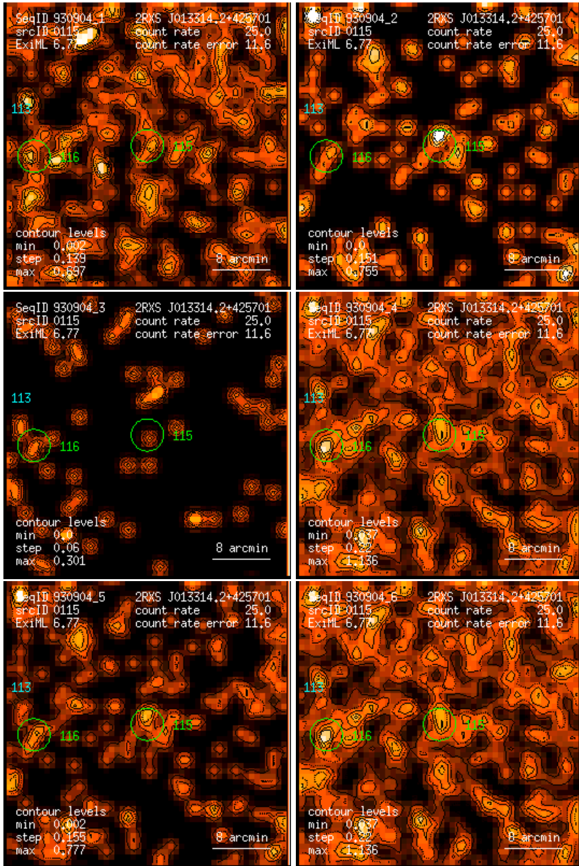
Figure 115: RASS 930904: detection 0115: band rate images, Gaussian filter: (1) PSPC channels 11 – 41, (2) 52 – 90, (3) 91 – 201, (4) 11 – 235, (5) 52 – 201, (6) 11 – 201. Broad band rates in counts/ks. Band rate contour levels in counts/ks/arcmin 2 .
