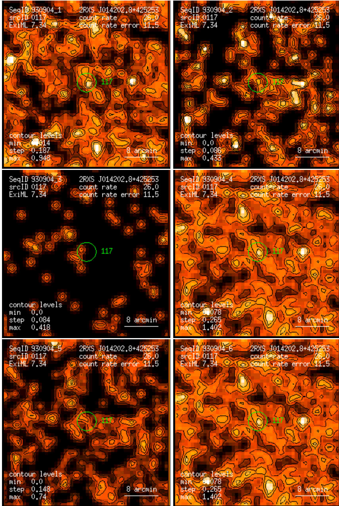
Figure 117: RASS 930904: detection 0117: band rate images, Gaussian filter: (1) PSPC channels 11 – 41, (2) 52 – 90, (3) 91 – 201, (4) 11 – 235, (5) 52 – 201, (6) 11 – 201. Broad band rates in counts/ks. Band rate contour levels in counts/ks/arcmin 2 .
