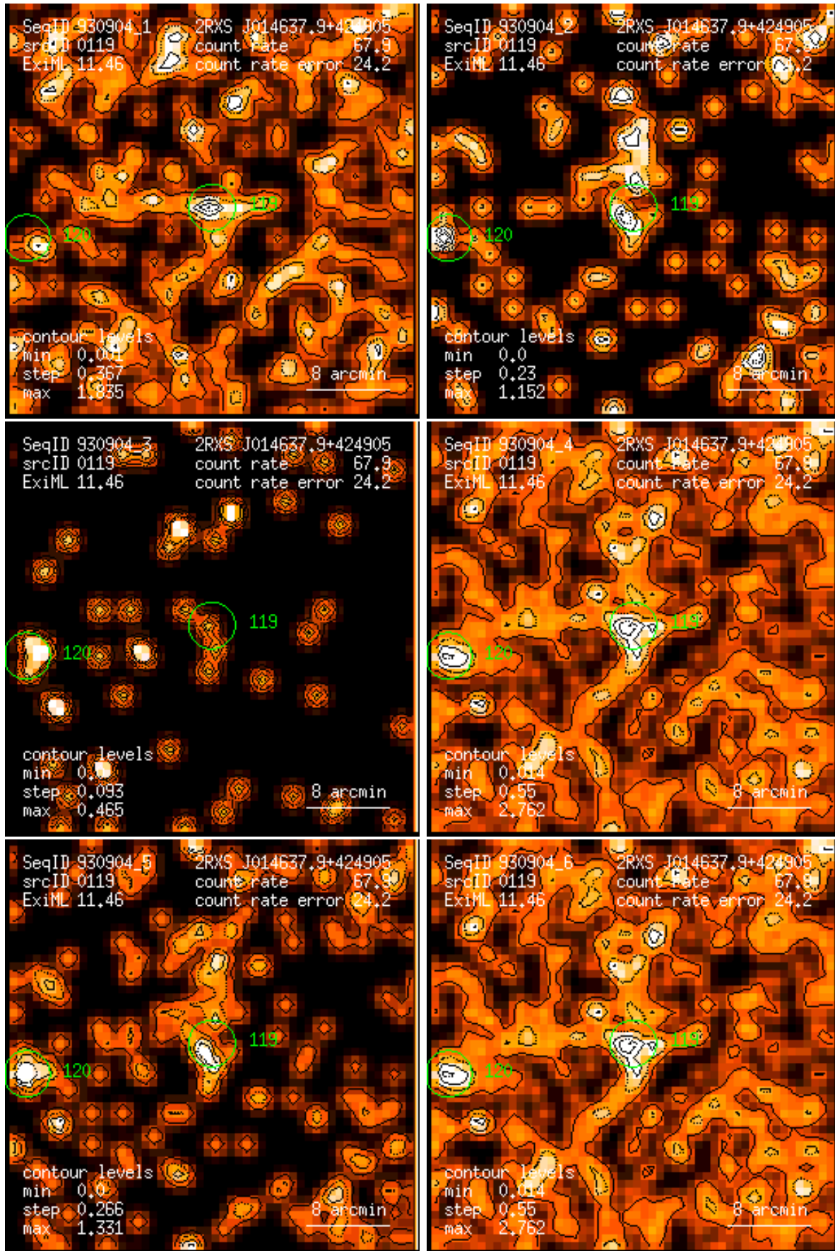
Figure 119: RASS 930904: detection 0119: band rate images, Gaussian filter: (1) PSPC channels 11 – 41, (2) 52 – 90, (3) 91 – 201, (4) 11 – 235, (5) 52 – 201, (6) 11 – 201. Broad band rates in counts/ks. Band rate contour levels in counts/ks/arcmin 2 .
