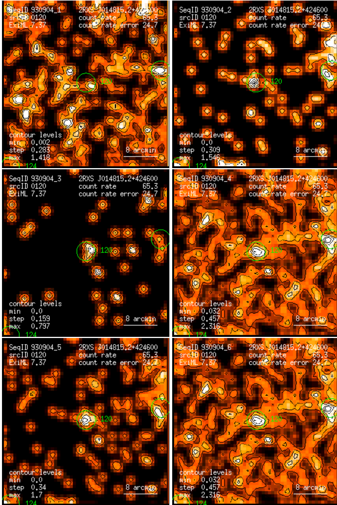
Figure 120: RASS 930904: detection 0120: band rate images, Gaussian filter: (1) PSPC channels 11 – 41, (2) 52 – 90, (3) 91 – 201, (4) 11 – 235, (5) 52 – 201, (6) 11 – 201. Broad band rates in counts/ks. Band rate contour levels in counts/ks/arcmin 2 .
