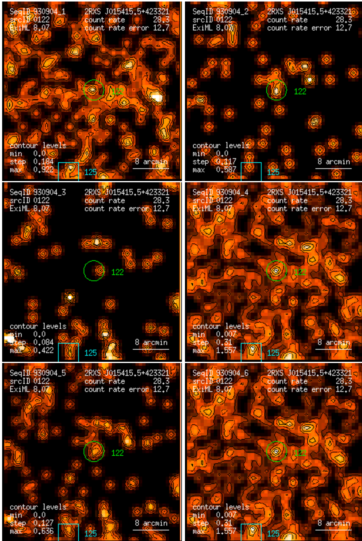
Figure 122: RASS 930904: detection 0122: band rate images, Gaussian filter: (1) PSPC channels 11 – 41, (2) 52 – 90, (3) 91 – 201, (4) 11 – 235, (5) 52 – 201, (6) 11 – 201. Broad band rates in counts/ks. Band rate contour levels in counts/ks/arcmin 2 .
