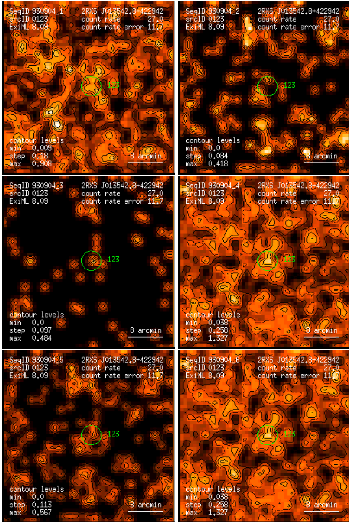
Figure 123: RASS 930904: detection 0123: band rate images, Gaussian filter: (1) PSPC channels 11 – 41, (2) 52 – 90, (3) 91 – 201, (4) 11 – 235, (5) 52 – 201, (6) 11 – 201. Broad band rates in counts/ks. Band rate contour levels in counts/ks/arcmin 2 .
