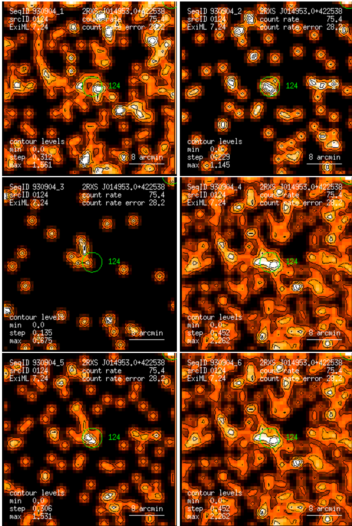
Figure 124: RASS 930904: detection 0124: band rate images, Gaussian filter: (1) PSPC channels 11 – 41, (2) 52 – 90, (3) 91 – 201, (4) 11 – 235, (5) 52 – 201, (6) 11 – 201. Broad band rates in counts/ks. Band rate contour levels in counts/ks/arcmin 2 .
