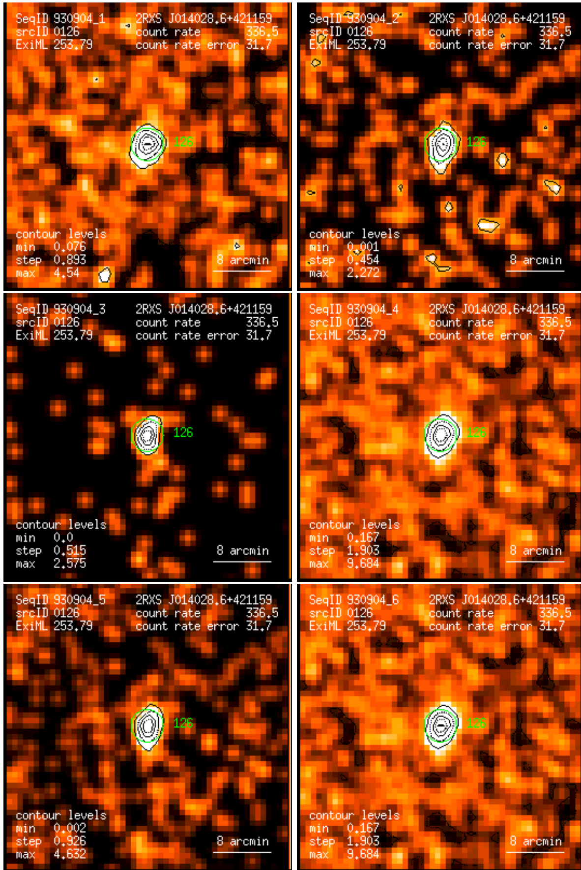
Figure 126: RASS 930904: detection 0126: band rate images, Gaussian filter: (1) PSPC channels 11 – 41, (2) 52 – 90, (3) 91 – 201, (4) 11 – 235, (5) 52 – 201, (6) 11 – 201. Broad band rates in counts/ks. Band rate contour levels in counts/ks/arcmin 2 .
