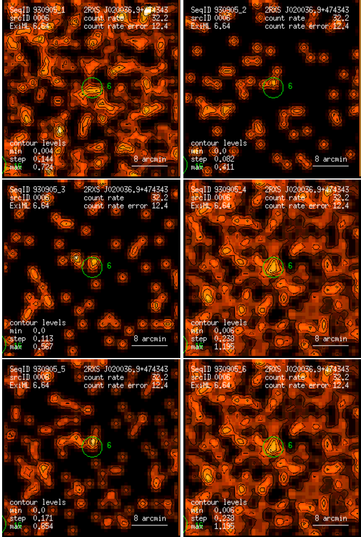
Figure 6: RASS 930905: detection 0006: band rate images, Gaussian filter: (1) PSPC channels 11 – 41, (2) 52 – 90, (3) 91 – 201, (4) 11 – 235, (5) 52 – 201, (6) 11 – 201. Broad band rates in counts/ks. Band rate contour levels in counts/ks/arcmin 2 .
