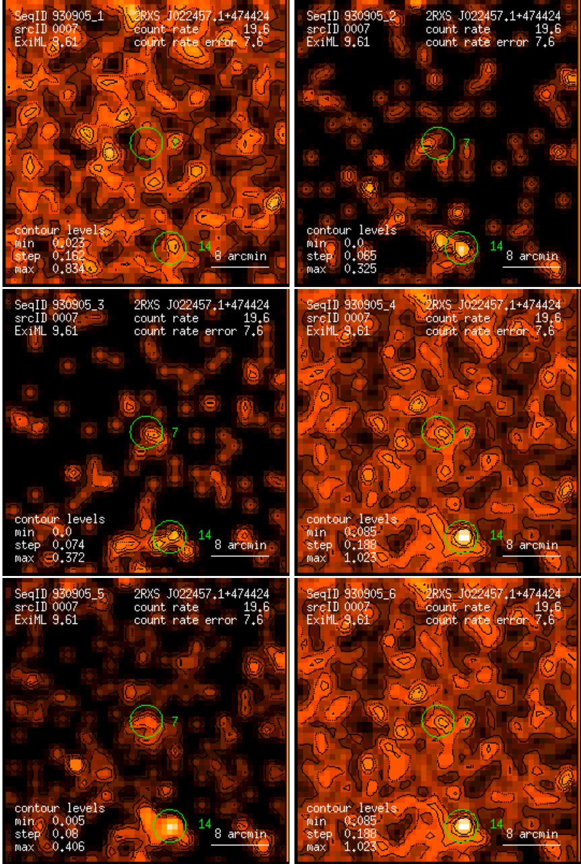
Figure 7: RASS 930905: detection 0007: band rate images, Gaussian filter: (1) PSPC channels 11 – 41, (2) 52 – 90, (3) 91 – 201, (4) 11 – 235, (5) 52 – 201, (6) 11 – 201. Broad band rates in counts/ks. Band rate contour levels in counts/ks/arcmin 2 .
