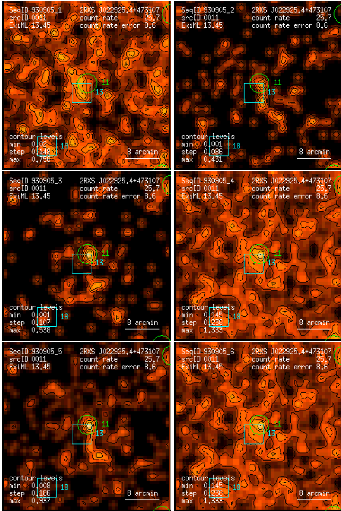
Figure 11: RASS 930905: detection 0011: band rate images, Gaussian filter: (1) PSPC channels 11 – 41, (2) 52 – 90, (3) 91 – 201, (4) 11 – 235, (5) 52 – 201, (6) 11 – 201. Broad band rates in counts/ks. Band rate contour levels in counts/ks/arcmin 2 .
