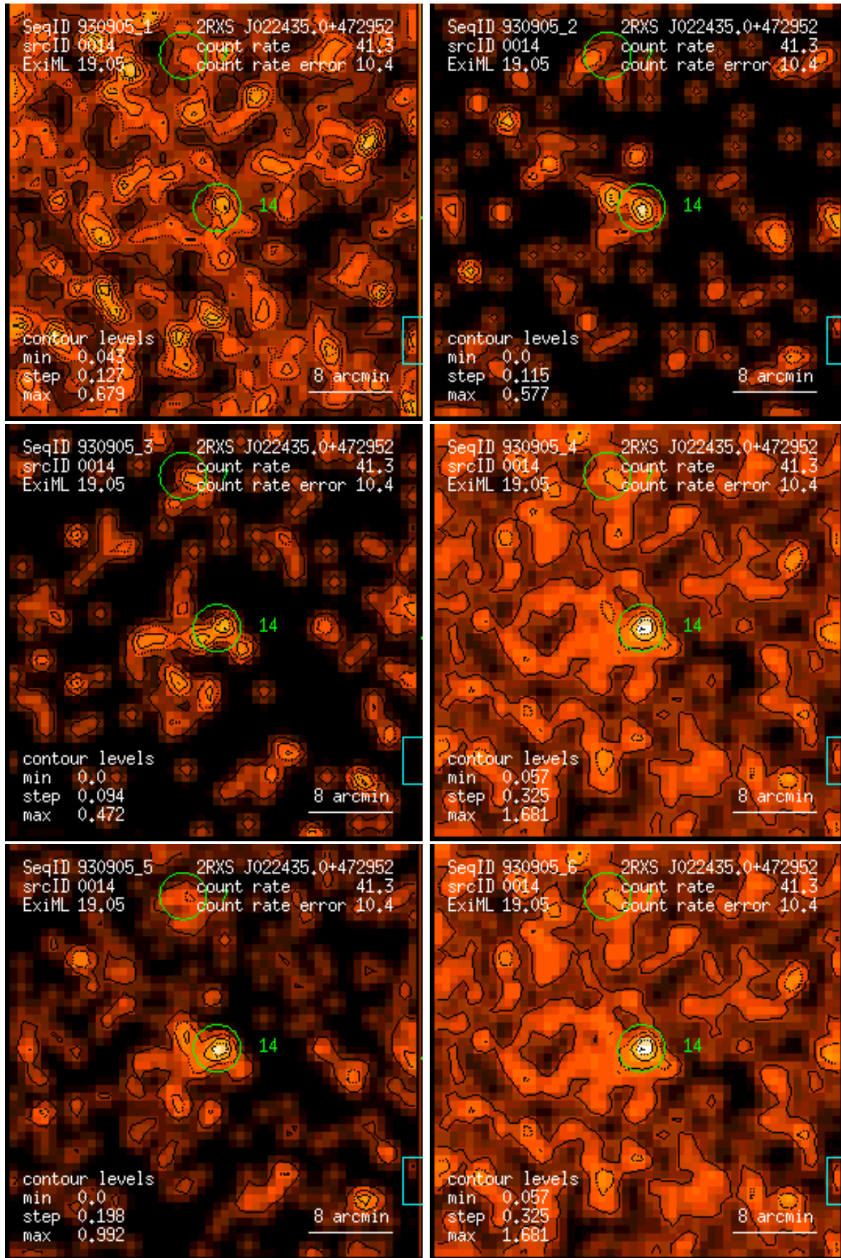
Figure 14: RASS 930905: detection 0014: band rate images, Gaussian filter: (1) PSPC channels 11 – 41, (2) 52 – 90, (3) 91 – 201, (4) 11 – 235, (5) 52 – 201, (6) 11 – 201. Broad band rates in counts/ks. Band rate contour levels in counts/ks/arcmin 2 .
