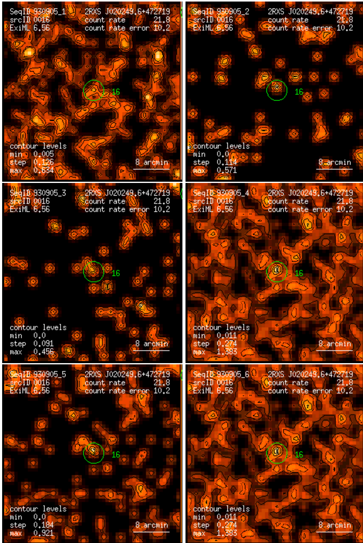
Figure 16: RASS 930905: detection 0016: band rate images, Gaussian filter: (1) PSPC channels 11 – 41, (2) 52 – 90, (3) 91 – 201, (4) 11 – 235, (5) 52 – 201, (6) 11 – 201. Broad band rates in counts/ks. Band rate contour levels in counts/ks/arcmin 2 .
