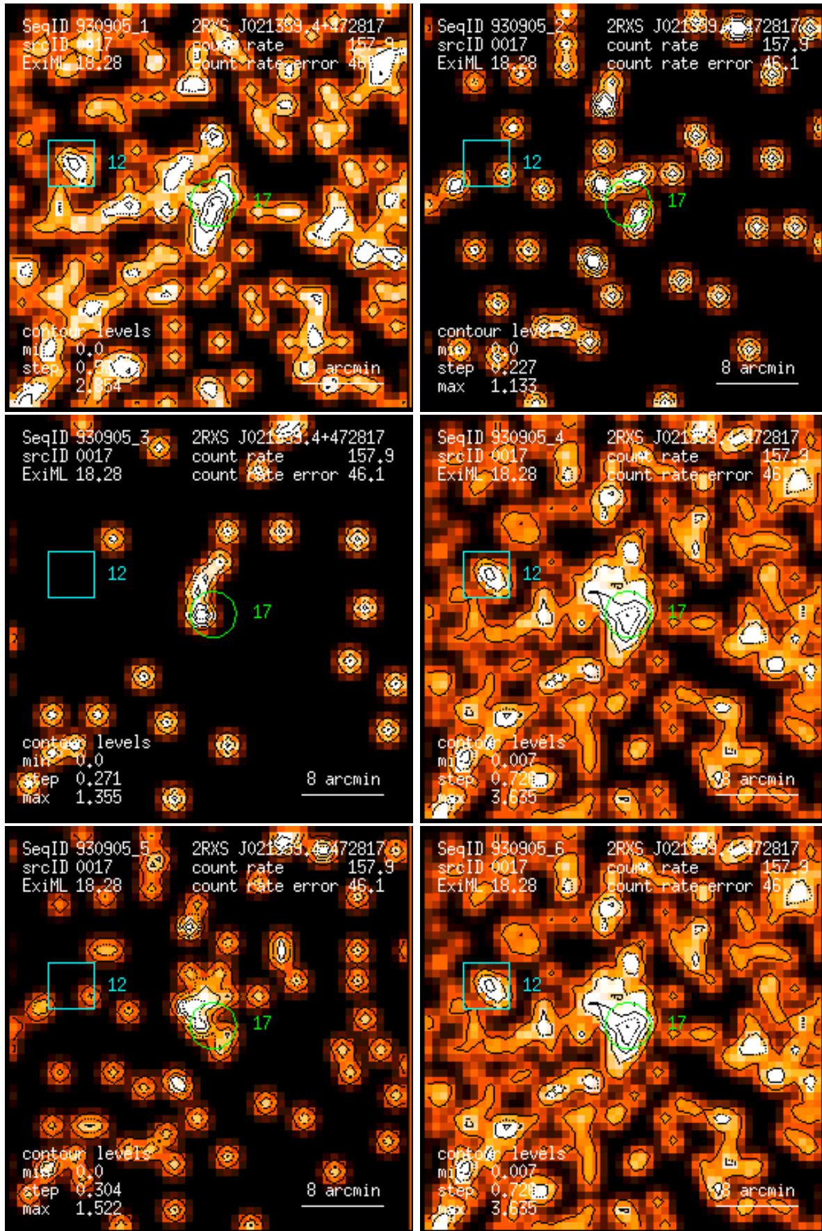
Figure 17: RASS 930905: detection 0017: band rate images, Gaussian filter: (1) PSPC channels 11 – 41, (2) 52 – 90, (3) 91 – 201, (4) 11 – 235, (5) 52 – 201, (6) 11 – 201. Broad band rates in counts/ks. Band rate contour levels in counts/ks/arcmin 2 .
