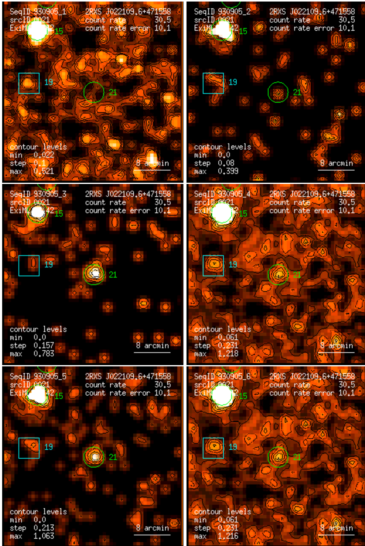
Figure 21: RASS 930905: detection 0021: band rate images, Gaussian filter: (1) PSPC channels 11 – 41, (2) 52 – 90, (3) 91 – 201, (4) 11 – 235, (5) 52 – 201, (6) 11 – 201. Broad band rates in counts/ks. Band rate contour levels in counts/ks/arcmin 2 .
