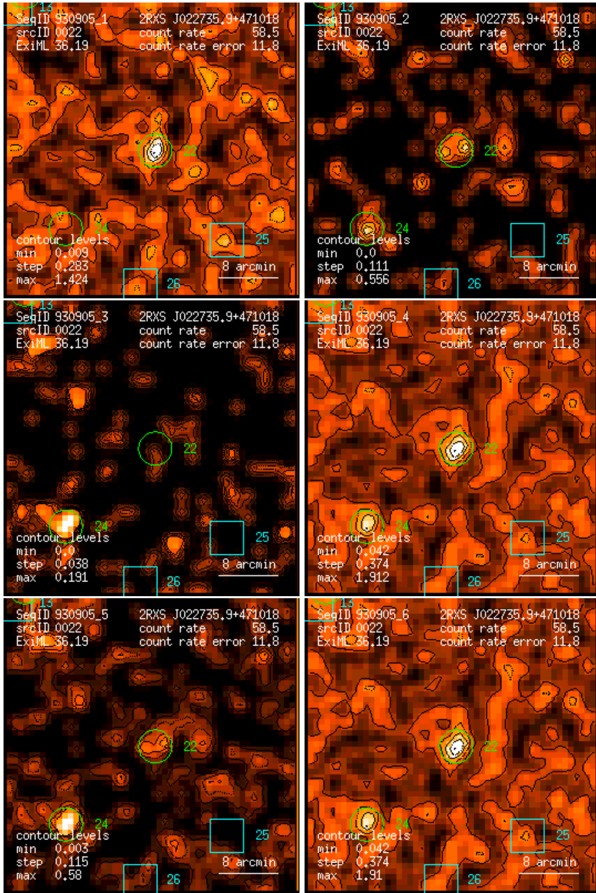
Figure 22: RASS 930905: detection 0022: band rate images, Gaussian filter: (1) PSPC channels 11 – 41, (2) 52 – 90, (3) 91 – 201, (4) 11 – 235, (5) 52 – 201, (6) 11 – 201. Broad band rates in counts/ks. Band rate contour levels in counts/ks/arcmin 2 .
