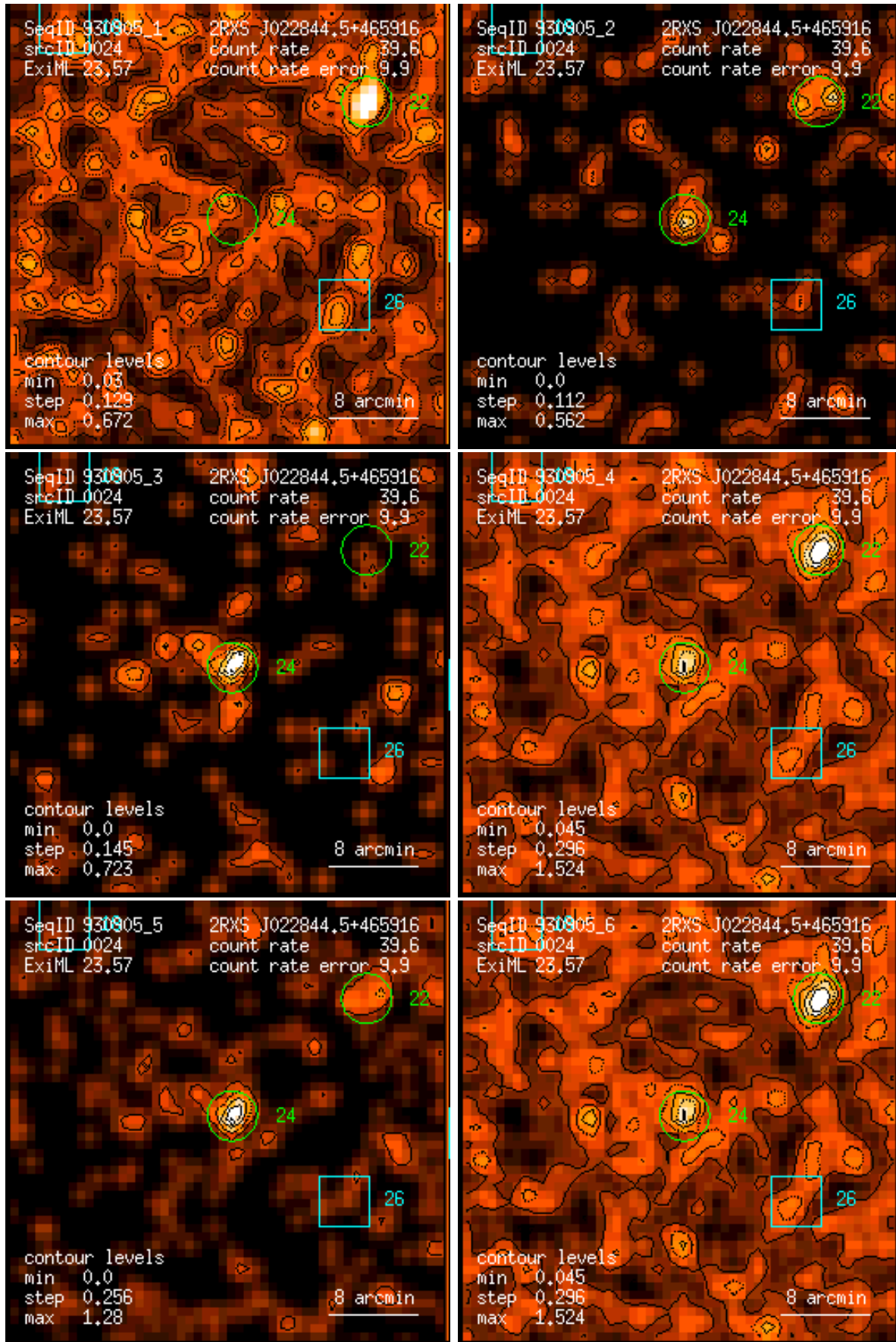
Figure 24: RASS 930905: detection 0024: band rate images, Gaussian filter: (1) PSPC channels 11 – 41, (2) 52 – 90, (3) 91 – 201, (4) 11 – 235, (5) 52 – 201, (6) 11 – 201. Broad band rates in counts/ks. Band rate contour levels in counts/ks/arcmin 2 .
