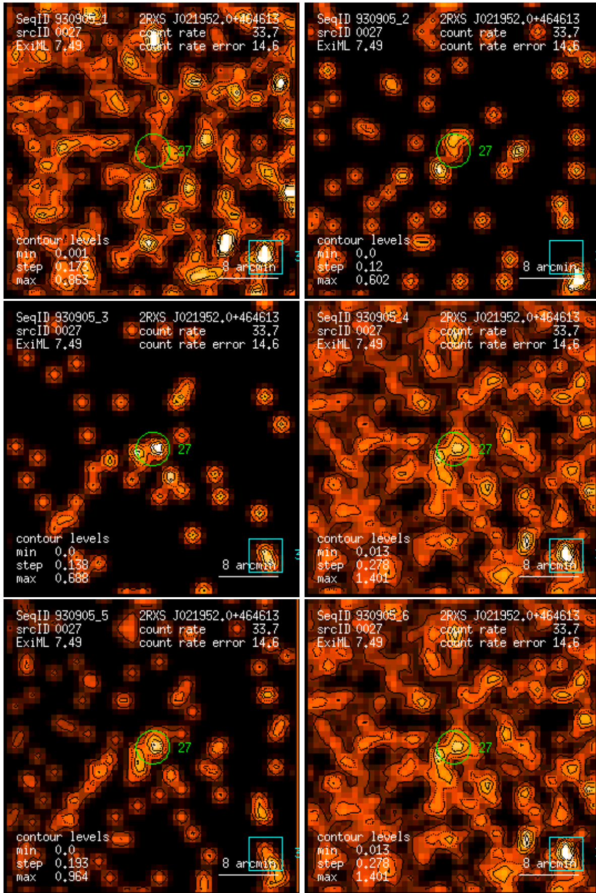
Figure 27: RASS 930905: detection 0027: band rate images, Gaussian filter: (1) PSPC channels 11 – 41, (2) 52 – 90, (3) 91 – 201, (4) 11 – 235, (5) 52 – 201, (6) 11 – 201. Broad band rates in counts/ks. Band rate contour levels in counts/ks/arcmin 2 .
