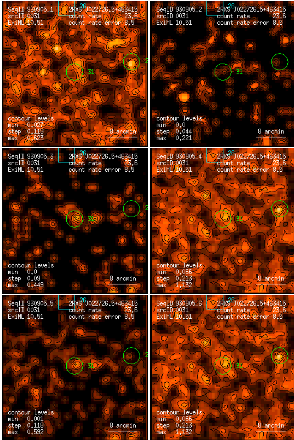
Figure 31: RASS 930905: detection 0031: band rate images, Gaussian filter: (1) PSPC channels 11 – 41, (2) 52 – 90, (3) 91 – 201, (4) 11 – 235, (5) 52 – 201, (6) 11 – 201. Broad band rates in counts/ks. Band rate contour levels in counts/ks/arcmin 2 .
