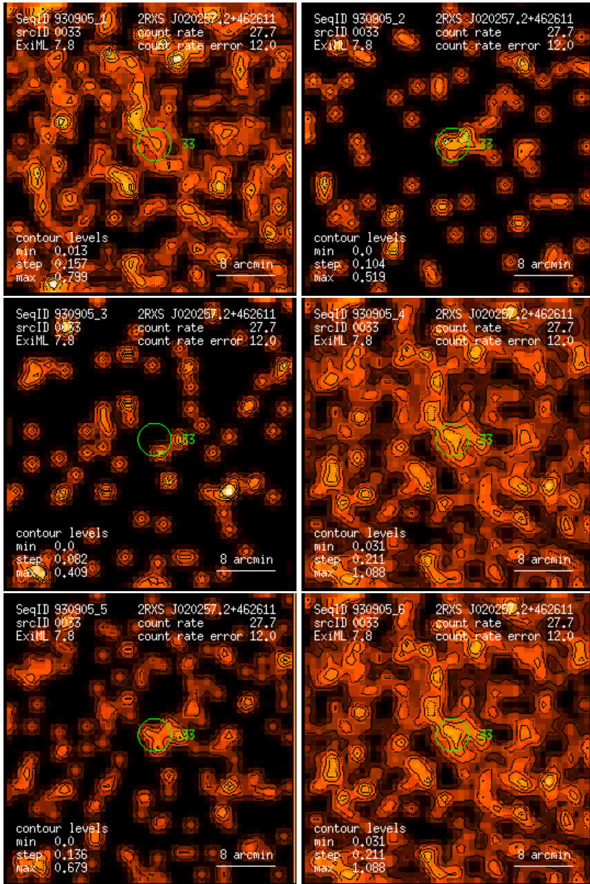
Figure 33: RASS 930905: detection 0033: band rate images, Gaussian filter: (1) PSPC channels 11 – 41, (2) 52 – 90, (3) 91 – 201, (4) 11 – 235, (5) 52 – 201, (6) 11 – 201. Broad band rates in counts/ks. Band rate contour levels in counts/ks/arcmin 2 .
