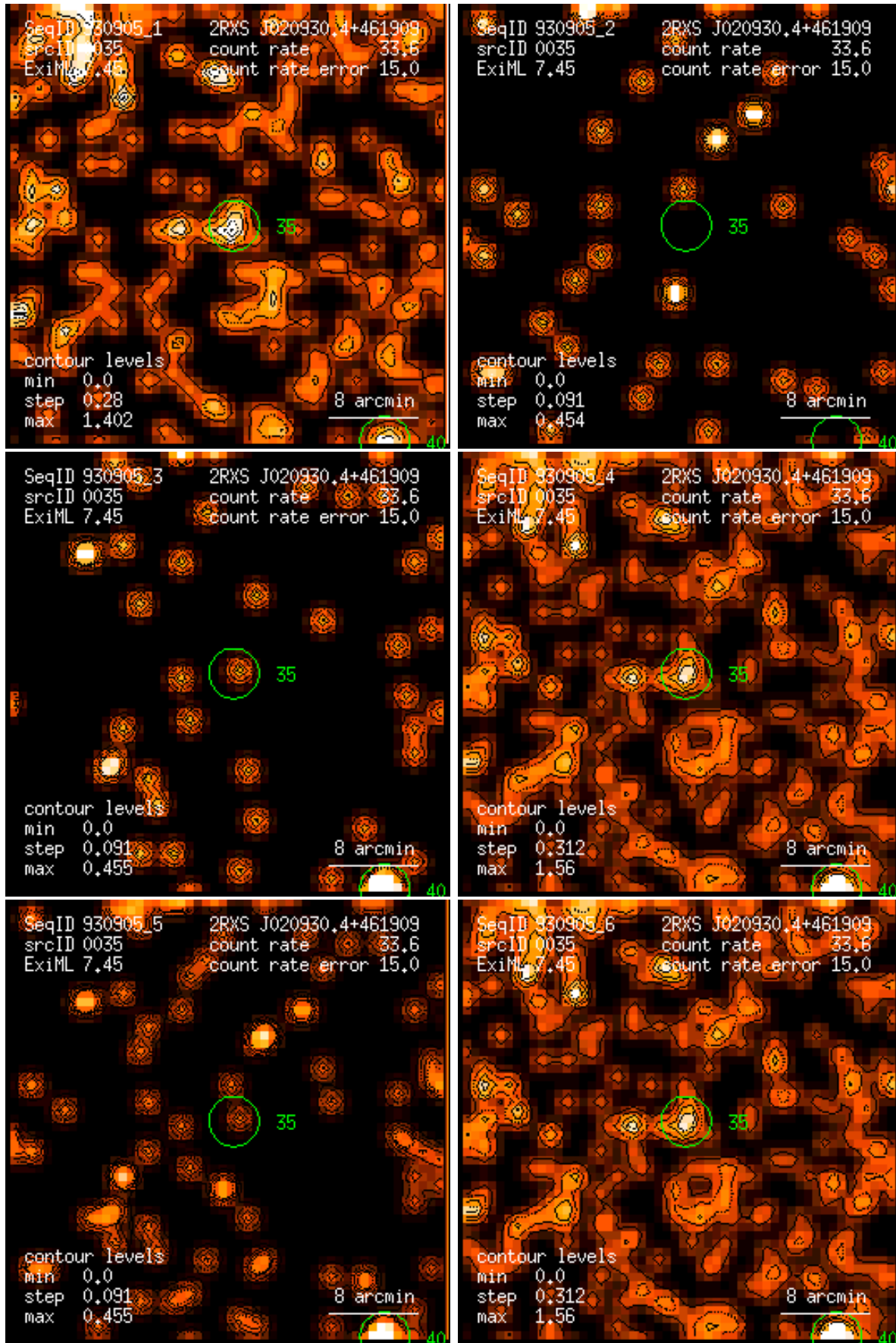
Figure 35: RASS 930905: detection 0035: band rate images, Gaussian filter: (1) PSPC channels 11 – 41, (2) 52 – 90, (3) 91 – 201, (4) 11 – 235, (5) 52 – 201, (6) 11 – 201. Broad band rates in counts/ks. Band rate contour levels in counts/ks/arcmin 2 .
