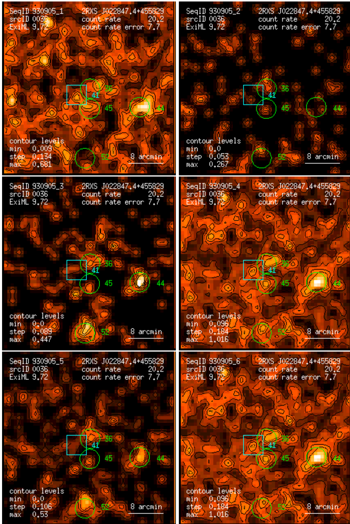
Figure 36: RASS 930905: detection 0036: band rate images, Gaussian filter: (1) PSPC channels 11 – 41, (2) 52 – 90, (3) 91 – 201, (4) 11 – 235, (5) 52 – 201, (6) 11 – 201. Broad band rates in counts/ks. Band rate contour levels in counts/ks/arcmin 2 .
