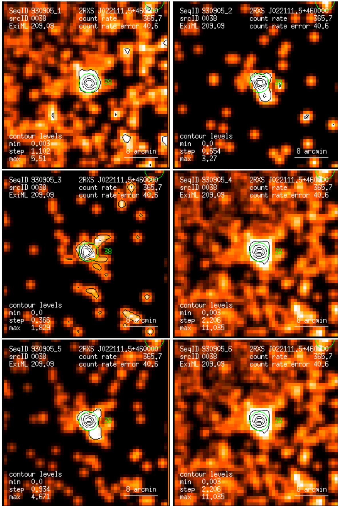
Figure 38: RASS 930905: detection 0038: band rate images, Gaussian filter: (1) PSPC channels 11 – 41, (2) 52 – 90, (3) 91 – 201, (4) 11 – 235, (5) 52 – 201, (6) 11 – 201. Broad band rates in counts/ks. Band rate contour levels in counts/ks/arcmin 2 .
