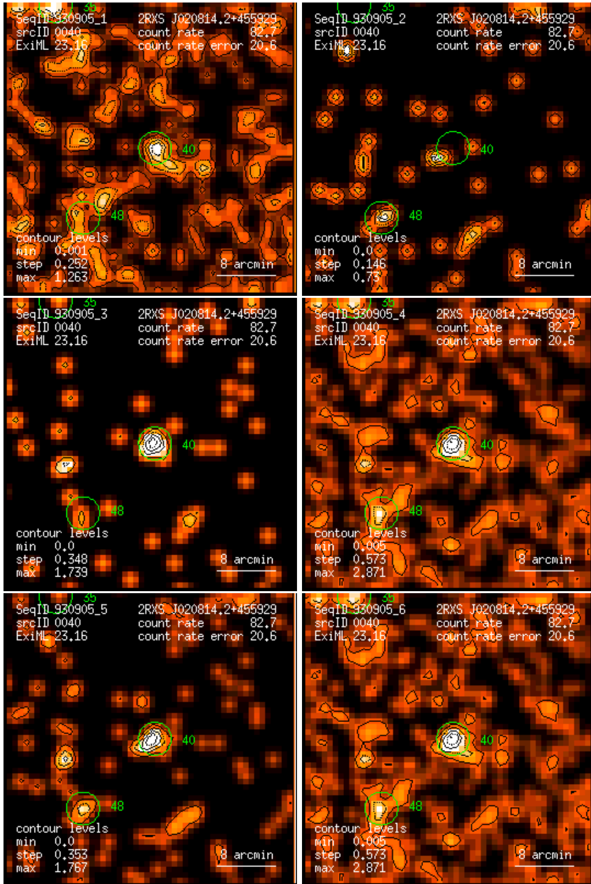
Figure 40: RASS 930905: detection 0040: band rate images, Gaussian filter: (1) PSPC channels 11 – 41, (2) 52 – 90, (3) 91 – 201, (4) 11 – 235, (5) 52 – 201, (6) 11 – 201. Broad band rates in counts/ks. Band rate contour levels in counts/ks/arcmin 2 .
