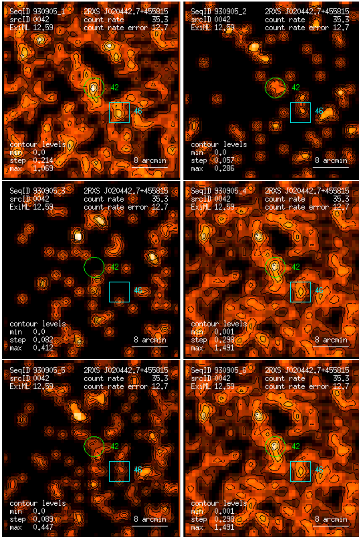
Figure 42: RASS 930905: detection 0042: band rate images, Gaussian filter: (1) PSPC channels 11 – 41, (2) 52 – 90, (3) 91 – 201, (4) 11 – 235, (5) 52 – 201, (6) 11 – 201. Broad band rates in counts/ks. Band rate contour levels in counts/ks/arcmin 2 .
