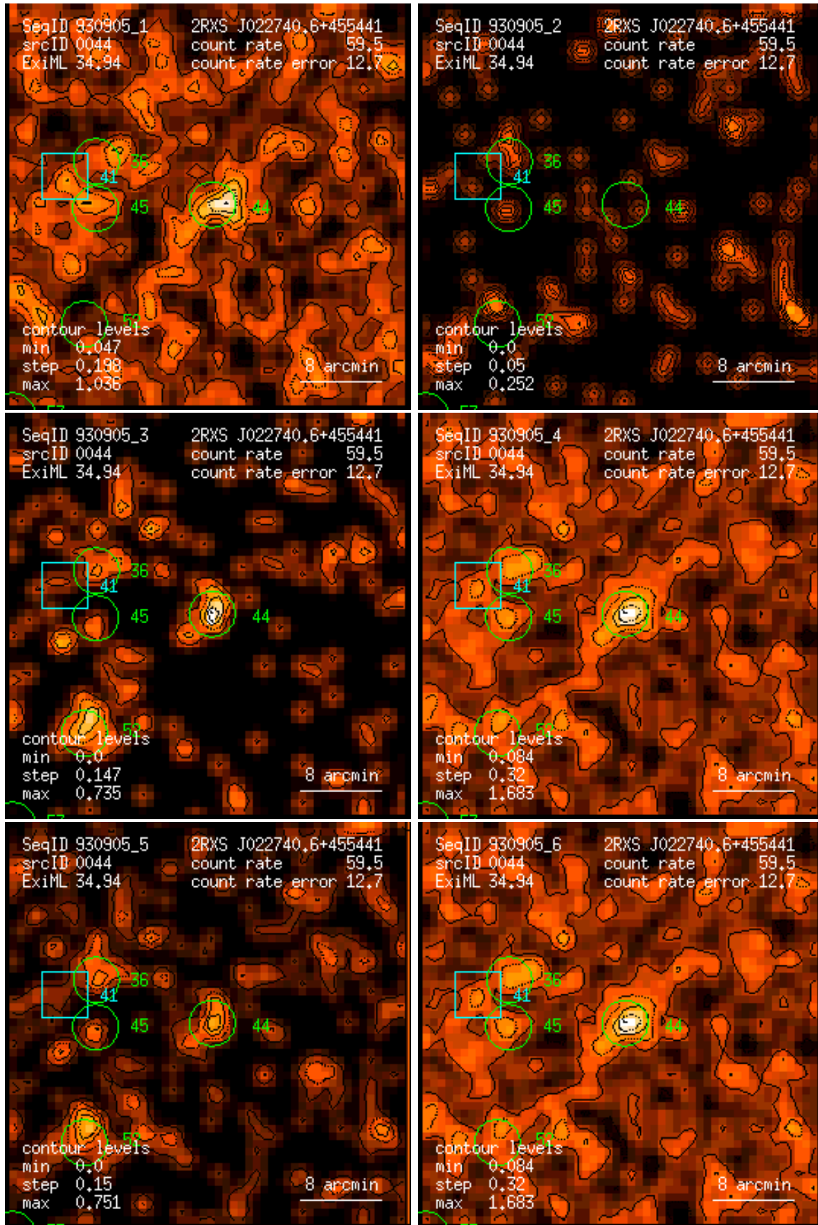
Figure 44: RASS 930905: detection 0044: band rate images, Gaussian filter: (1) PSPC channels 11 – 41, (2) 52 – 90, (3) 91 – 201, (4) 11 – 235, (5) 52 – 201, (6) 11 – 201. Broad band rates in counts/ks. Band rate contour levels in counts/ks/arcmin 2 .
