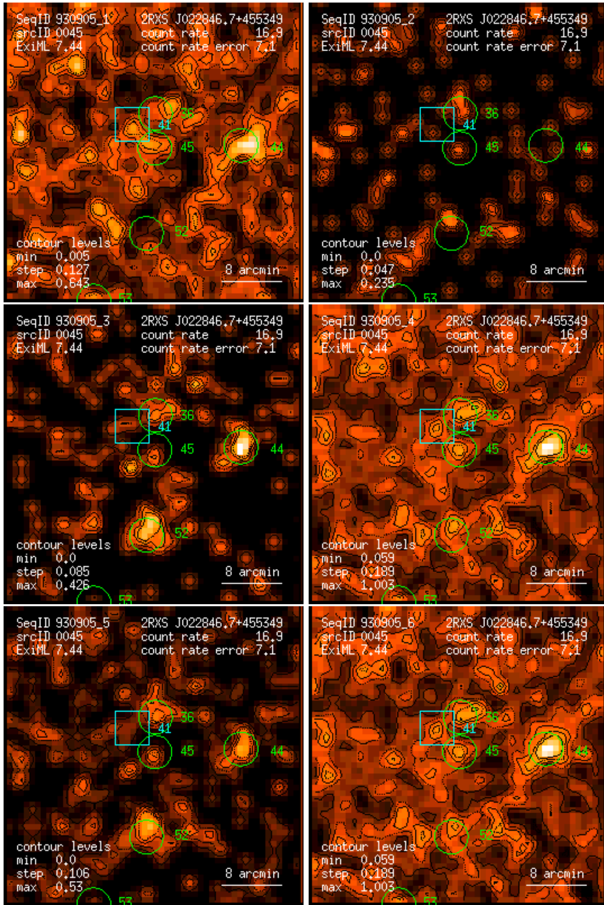
Figure 45: RASS 930905: detection 0045: band rate images, Gaussian filter: (1) PSPC channels 11 – 41, (2) 52 – 90, (3) 91 – 201, (4) 11 – 235, (5) 52 – 201, (6) 11 – 201. Broad band rates in counts/ks. Band rate contour levels in counts/ks/arcmin 2 .
