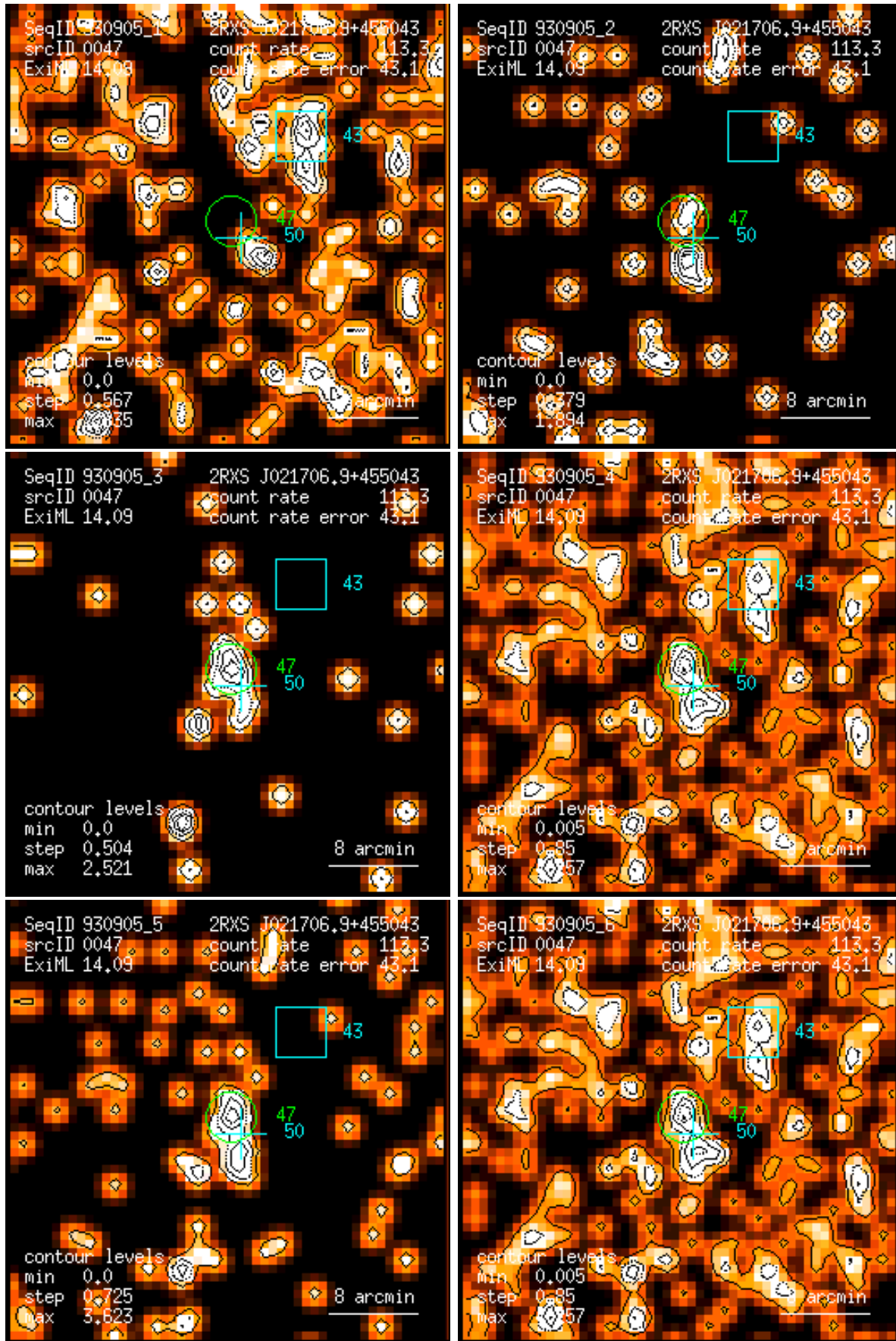
Figure 47: RASS 930905: detection 0047: band rate images, Gaussian filter: (1) PSPC channels 11 – 41, (2) 52 – 90, (3) 91 – 201, (4) 11 – 235, (5) 52 – 201, (6) 11 – 201. Broad band rates in counts/ks. Band rate contour levels in counts/ks/arcmin 2 .
