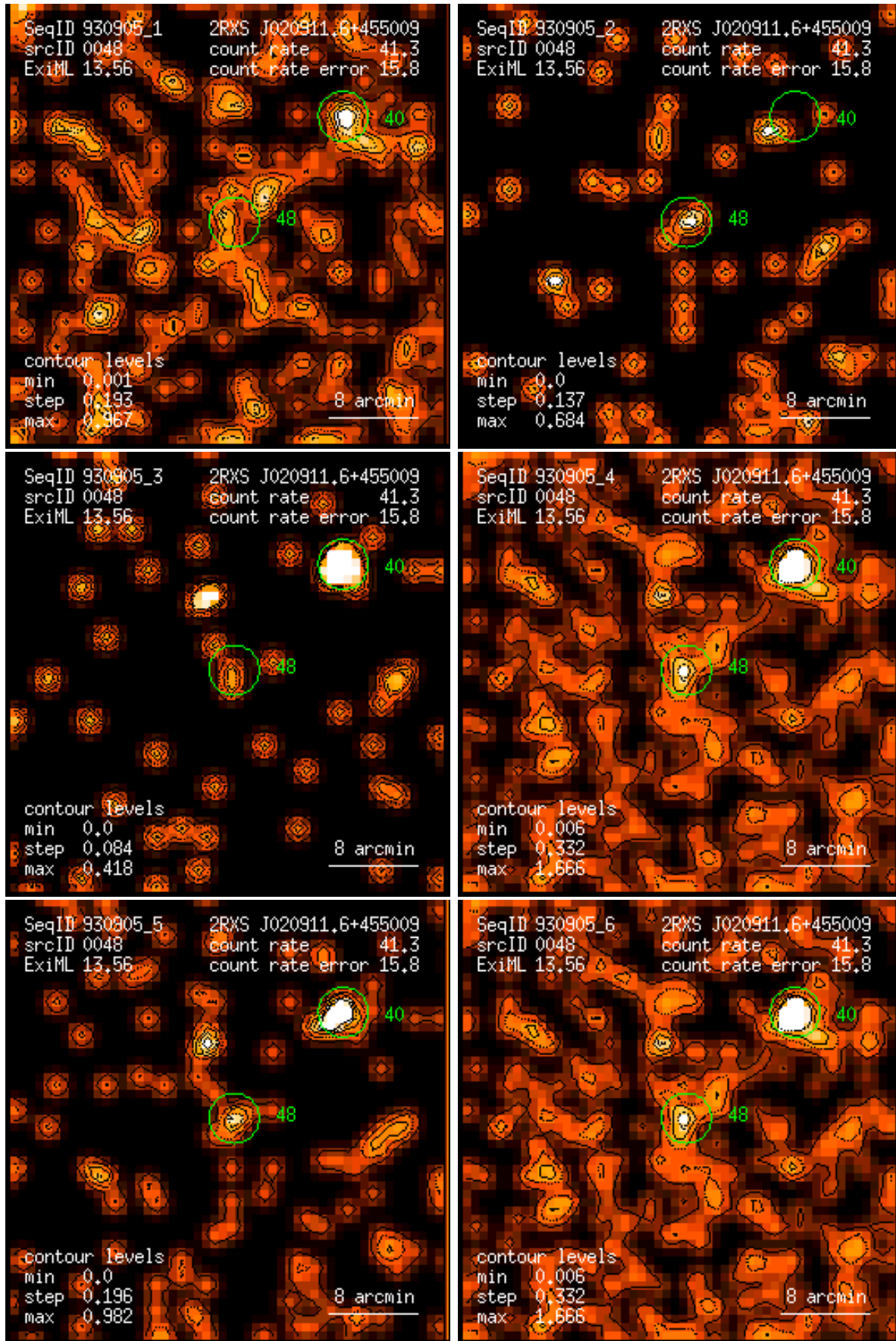
Figure 48: RASS 930905: detection 0048: band rate images, Gaussian filter: (1) PSPC channels 11 – 41, (2) 52 – 90, (3) 91 – 201, (4) 11 – 235, (5) 52 – 201, (6) 11 – 201. Broad band rates in counts/ks. Band rate contour levels in counts/ks/arcmin 2 .
