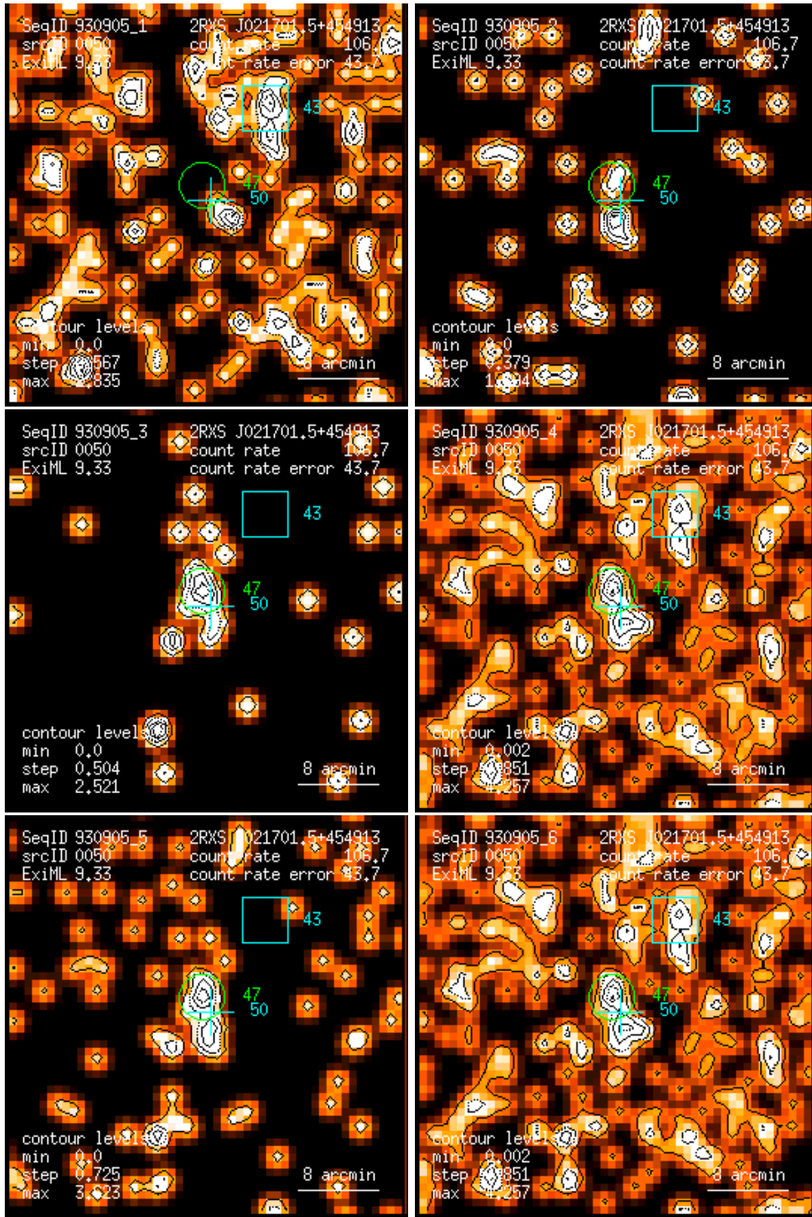
Figure 50: RASS 930905: detection 0050: band rate images, Gaussian filter: (1) PSPC channels 11 – 41, (2) 52 – 90, (3) 91 – 201, (4) 11 – 235, (5) 52 – 201, (6) 11 – 201. Broad band rates in counts/ks. Band rate contour levels in counts/ks/arcmin 2 .
