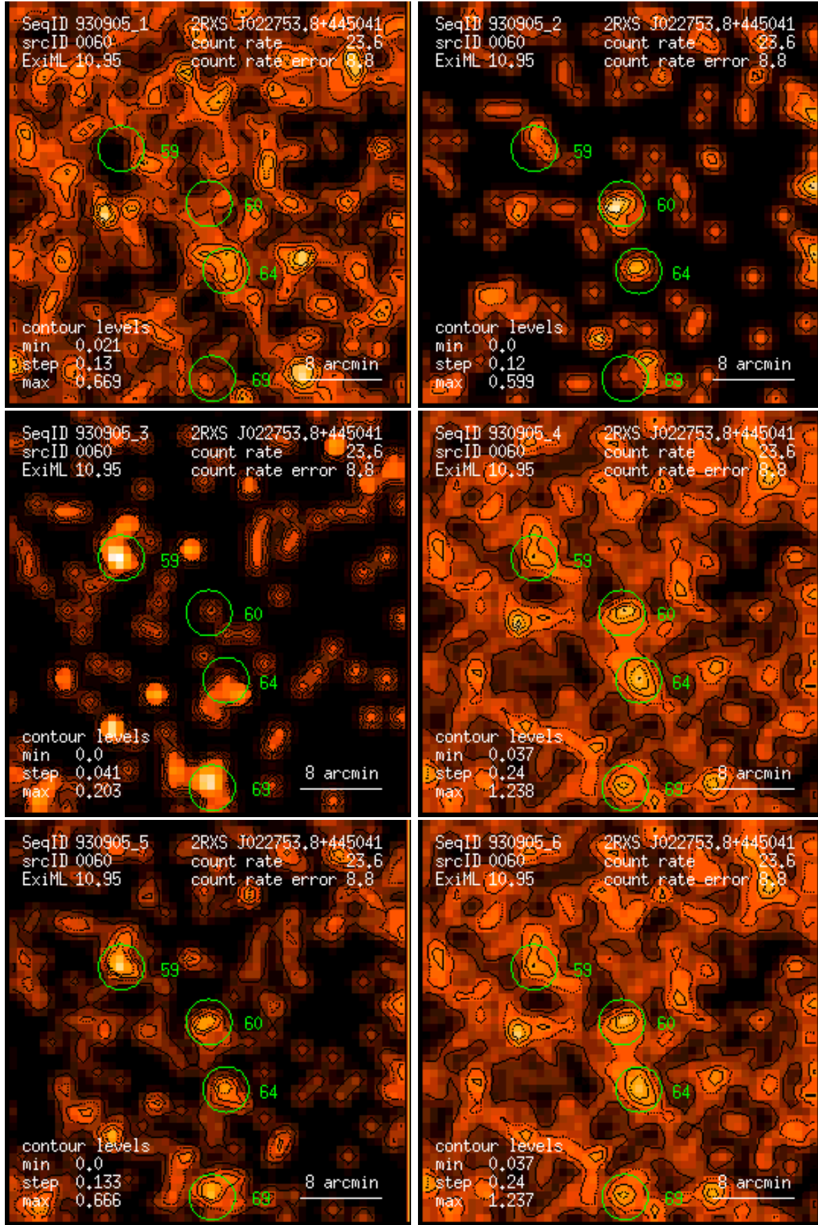
Figure 60: RASS 930905: detection 0060: band rate images, Gaussian filter: (1) PSPC channels 11 – 41, (2) 52 – 90, (3) 91 – 201, (4) 11 – 235, (5) 52 – 201, (6) 11 – 201. Broad band rates in counts/ks. Band rate contour levels in counts/ks/arcmin 2 .
