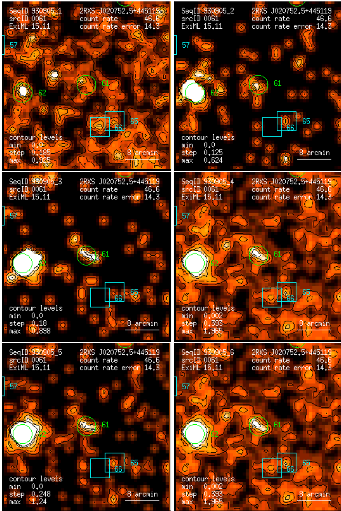
Figure 61: RASS 930905: detection 0061: band rate images, Gaussian filter: (1) PSPC channels 11 – 41, (2) 52 – 90, (3) 91 – 201, (4) 11 – 235, (5) 52 – 201, (6) 11 – 201. Broad band rates in counts/ks. Band rate contour levels in counts/ks/arcmin 2 .
