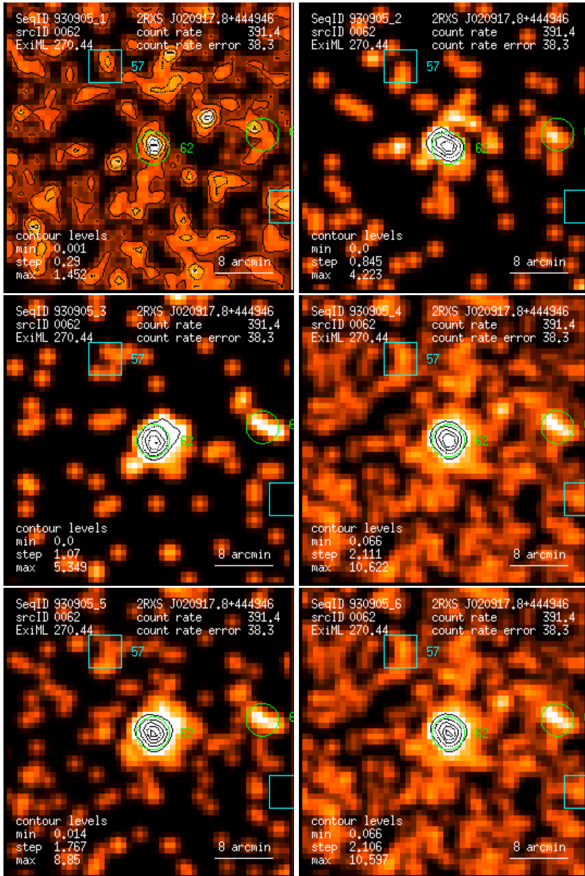
Figure 62: RASS 930905: detection 0062: band rate images, Gaussian filter: (1) PSPC channels 11 – 41, (2) 52 – 90, (3) 91 – 201, (4) 11 – 235, (5) 52 – 201, (6) 11 – 201. Broad band rates in counts/ks. Band rate contour levels in counts/ks/arcmin 2 .
