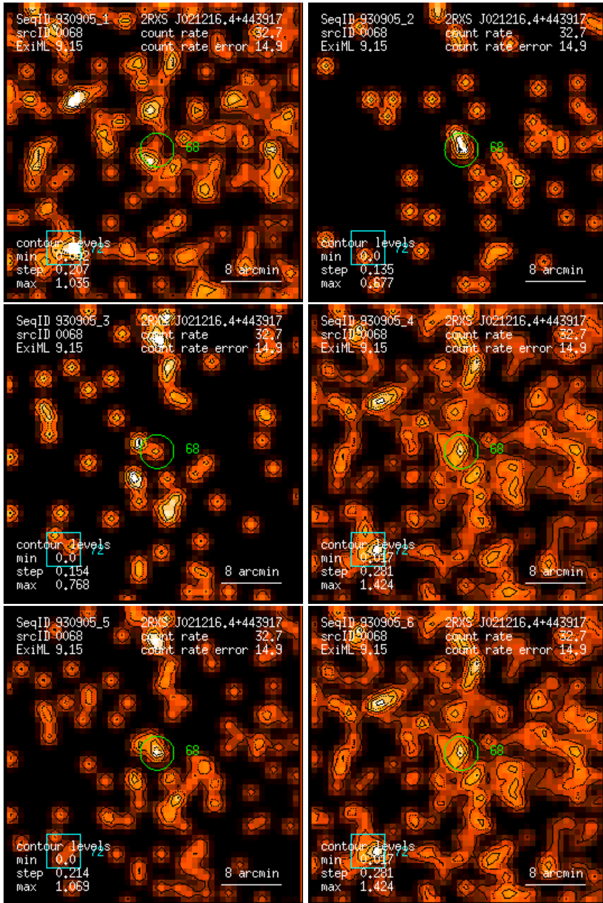
Figure 68: RASS 930905: detection 0068: band rate images, Gaussian filter: (1) PSPC channels 11 – 41, (2) 52 – 90, (3) 91 – 201, (4) 11 – 235, (5) 52 – 201, (6) 11 – 201. Broad band rates in counts/ks. Band rate contour levels in counts/ks/arcmin 2 .
